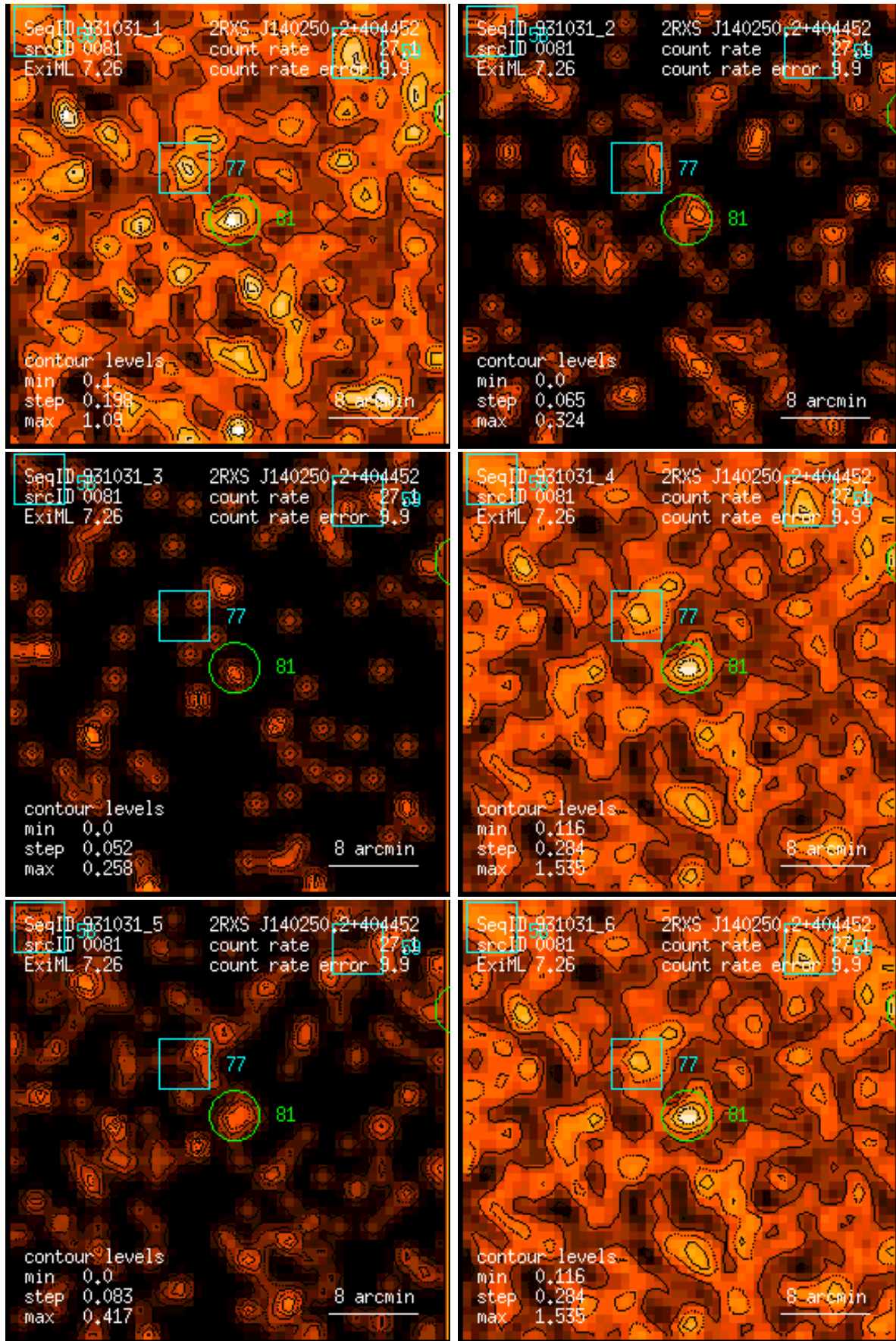
Figure 81: RASS 931031: detection 0081: band rate images, Gaussian filter: (1) PSPC channels 11 – 41, (2) 52 – 90, (3) 91 – 201, (4) 11 – 235, (5) 52 – 201, (6) 11 – 201. Broad band rates in counts/ks. Band rate contour levels in counts/ks/arcmin 2 .
