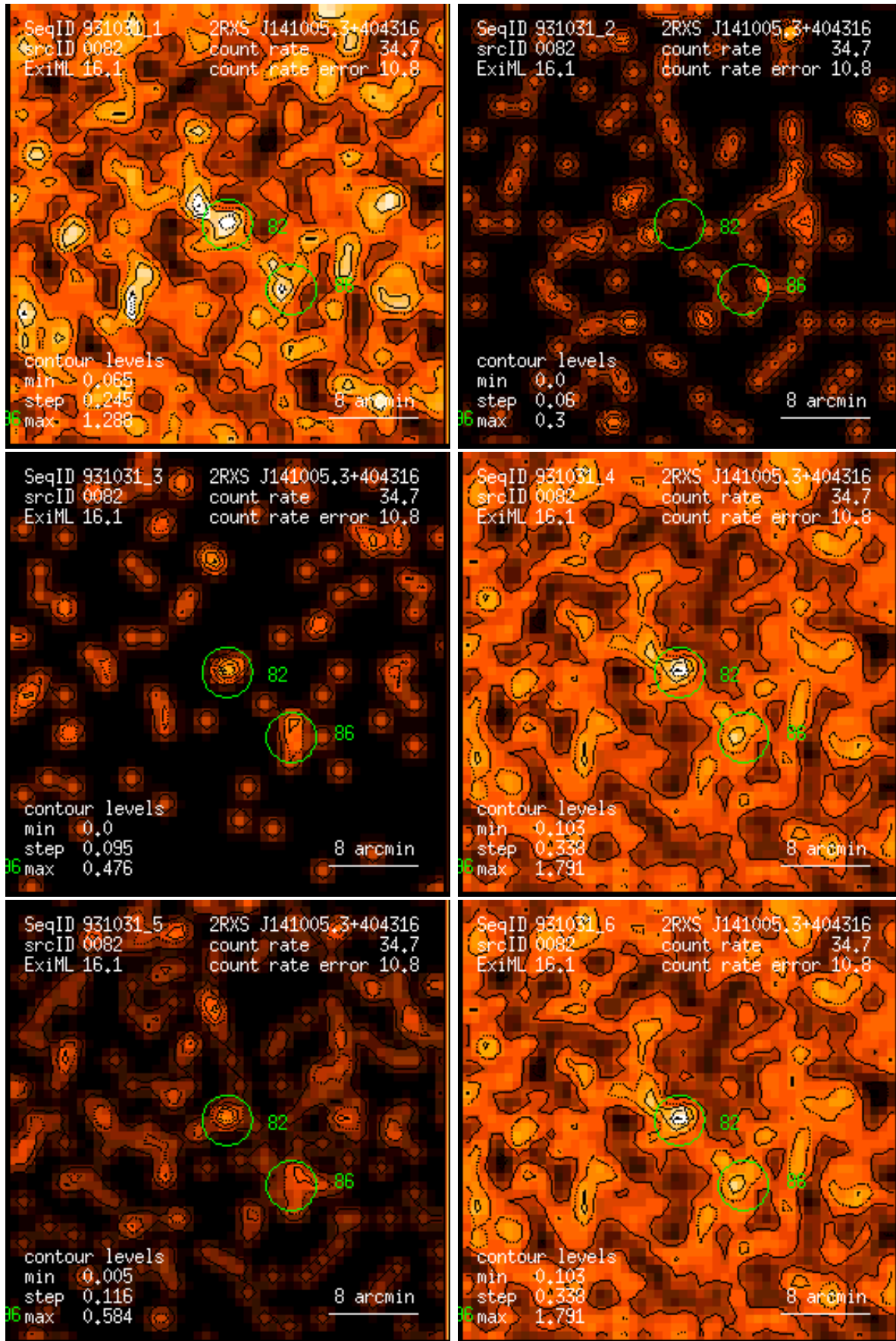
Figure 82: RASS 931031: detection 0082: band rate images, Gaussian filter: (1) PSPC channels 11 – 41, (2) 52 – 90, (3) 91 – 201, (4) 11 – 235, (5) 52 – 201, (6) 11 – 201. Broad band rates in counts/ks. Band rate contour levels in counts/ks/arcmin 2 .
