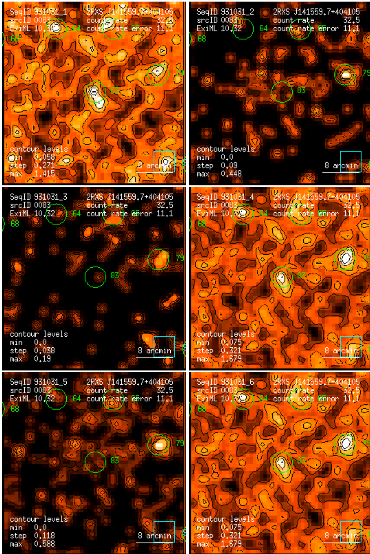
Figure 83: RASS 931031: detection 0083: band rate images, Gaussian filter: (1) PSPC channels 11 – 41, (2) 52 – 90, (3) 91 – 201, (4) 11 – 235, (5) 52 – 201, (6) 11 – 201. Broad band rates in counts/ks. Band rate contour levels in counts/ks/arcmin 2 .
