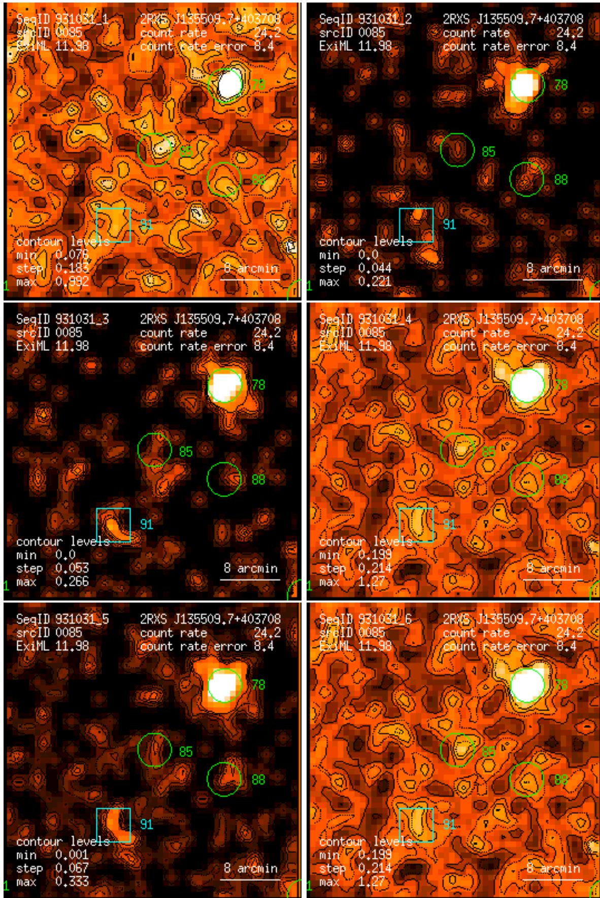
Figure 85: RASS 931031: detection 0085: band rate images, Gaussian filter: (1) PSPC channels 11 – 41, (2) 52 – 90, (3) 91 – 201, (4) 11 – 235, (5) 52 – 201, (6) 11 – 201. Broad band rates in counts/ks. Band rate contour levels in counts/ks/arcmin 2 .
