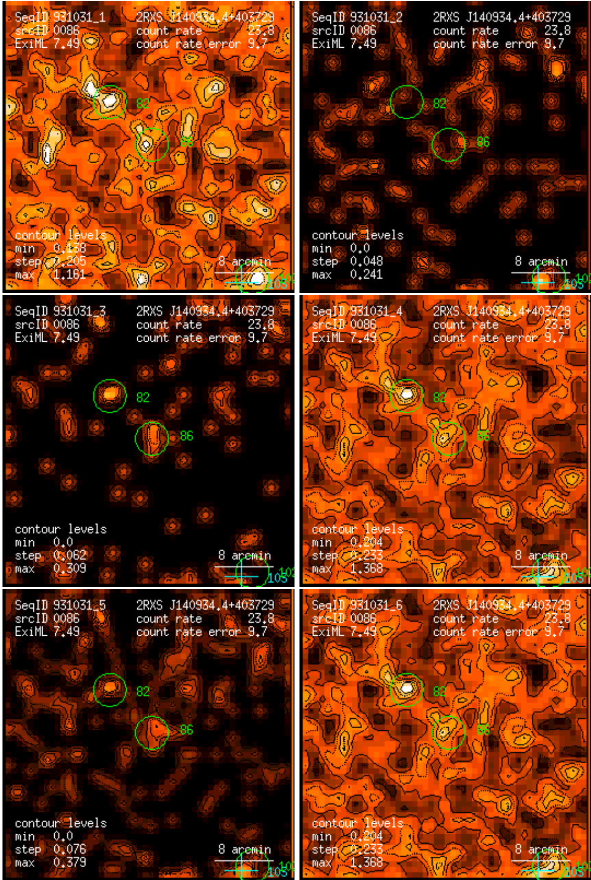
Figure 86: RASS 931031: detection 0086: band rate images, Gaussian filter: (1) PSPC channels 11 – 41, (2) 52 – 90, (3) 91 – 201, (4) 11 – 235, (5) 52 – 201, (6) 11 – 201. Broad band rates in counts/ks. Band rate contour levels in counts/ks/arcmin 2 .
