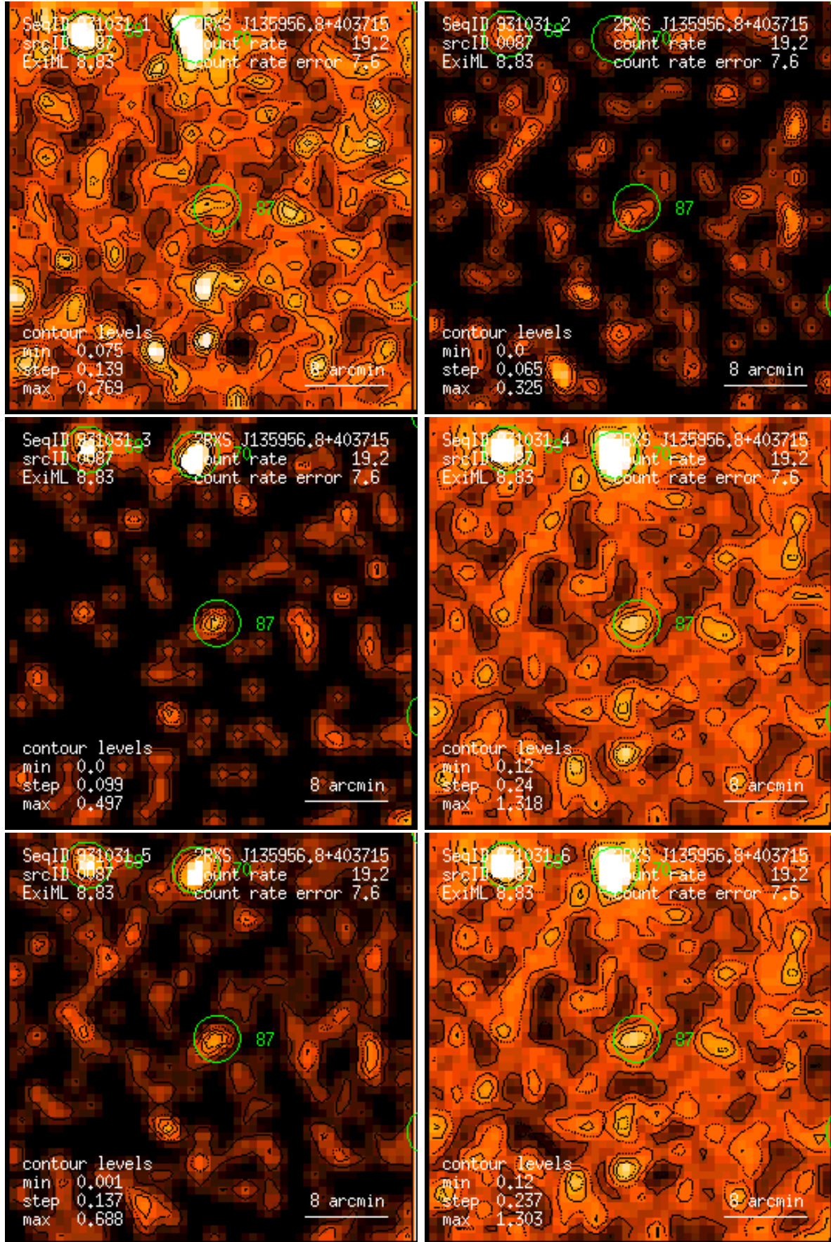
Figure 87: RASS 931031: detection 0087: band rate images, Gaussian filter: (1) PSPC channels 11 – 41, (2) 52 – 90, (3) 91 – 201, (4) 11 – 235, (5) 52 – 201, (6) 11 – 201. Broad band rates in counts/ks. Band rate contour levels in counts/ks/arcmin 2 .
