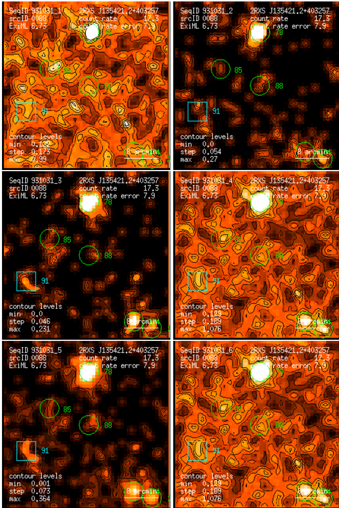
Figure 88: RASS 931031: detection 0088: band rate images, Gaussian filter: (1) PSPC channels 11 – 41, (2) 52 – 90, (3) 91 – 201, (4) 11 – 235, (5) 52 – 201, (6) 11 – 201. Broad band rates in counts/ks. Band rate contour levels in counts/ks/arcmin 2 .
