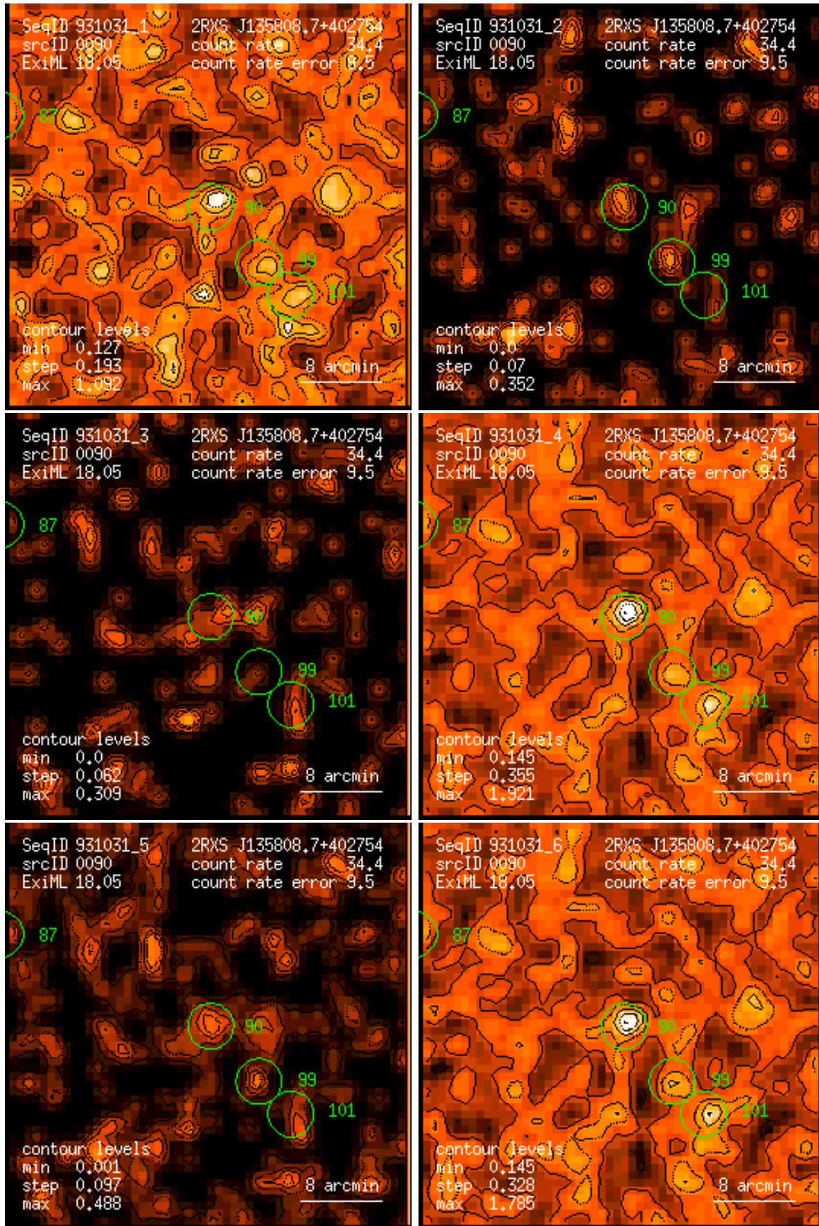
Figure 90: RASS 931031: detection 0090: band rate images, Gaussian filter: (1) PSPC channels 11 – 41, (2) 52 – 90, (3) 91 – 201, (4) 11 – 235, (5) 52 – 201, (6) 11 – 201. Broad band rates in counts/ks. Band rate contour levels in counts/ks/arcmin 2 .
