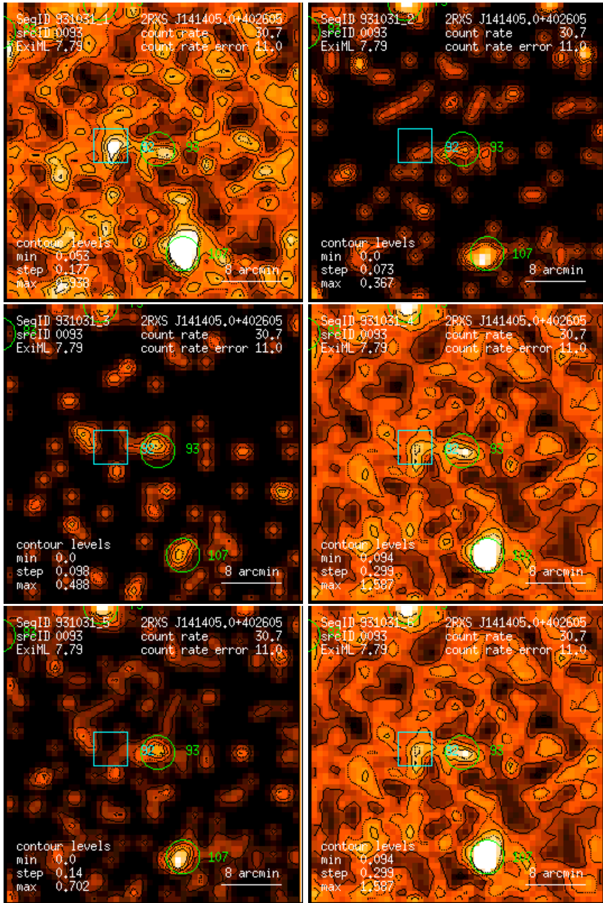
Figure 93: RASS 931031: detection 0093: band rate images, Gaussian filter: (1) PSPC channels 11 – 41, (2) 52 – 90, (3) 91 – 201, (4) 11 – 235, (5) 52 – 201, (6) 11 – 201. Broad band rates in counts/ks. Band rate contour levels in counts/ks/arcmin 2 .
