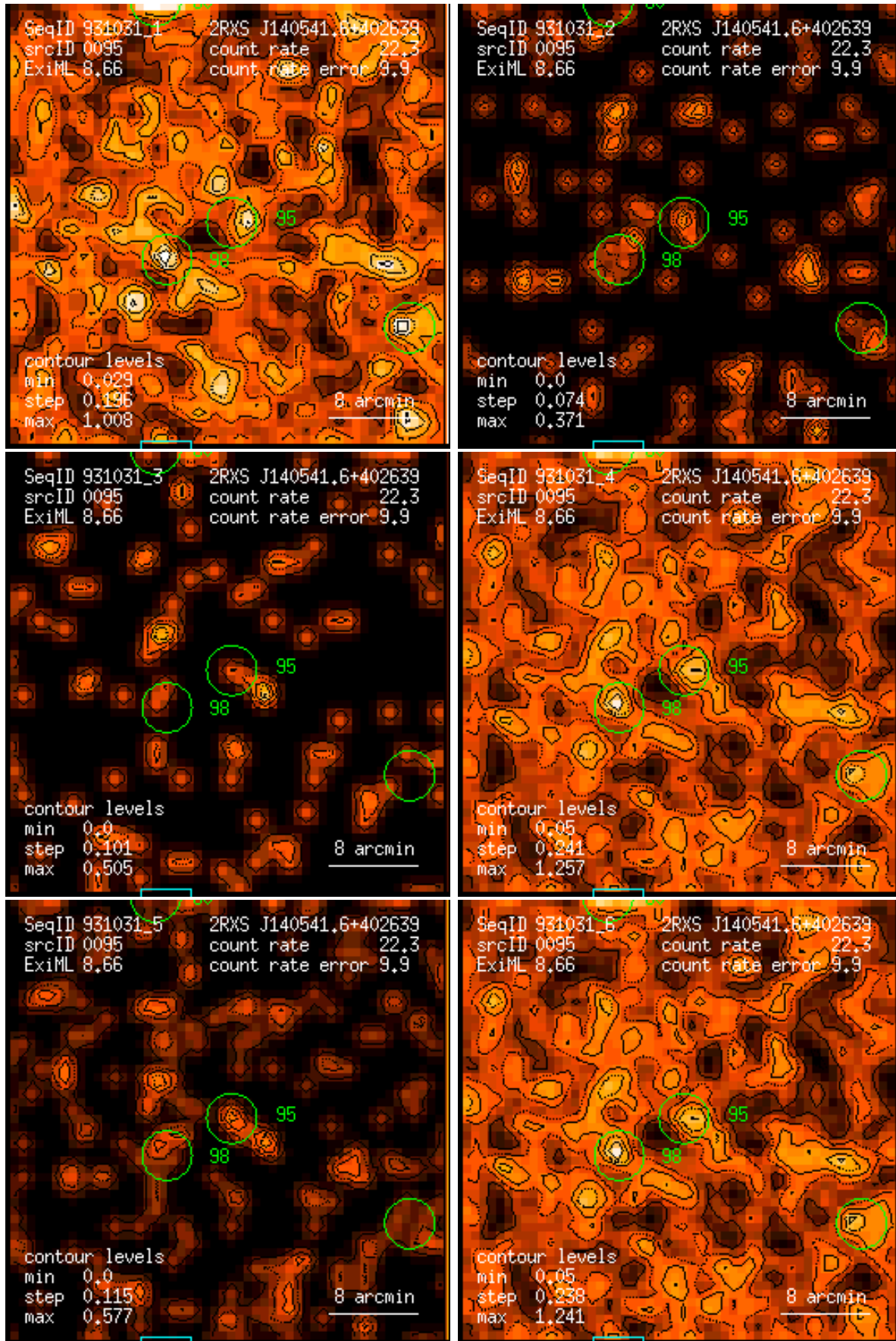
Figure 95: RASS 931031: detection 0095: band rate images, Gaussian filter: (1) PSPC channels 11 – 41, (2) 52 – 90, (3) 91 – 201, (4) 11 – 235, (5) 52 – 201, (6) 11 – 201. Broad band rates in counts/ks. Band rate contour levels in counts/ks/arcmin 2 .
