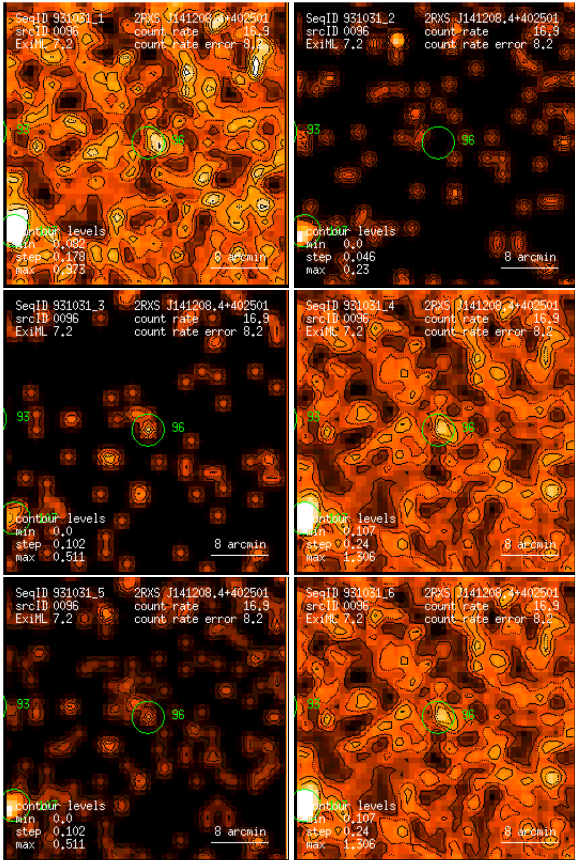
Figure 96: RASS 931031: detection 0096: band rate images, Gaussian filter: (1) PSPC channels 11 – 41, (2) 52 – 90, (3) 91 – 201, (4) 11 – 235, (5) 52 – 201, (6) 11 – 201. Broad band rates in counts/ks. Band rate contour levels in counts/ks/arcmin 2 .
