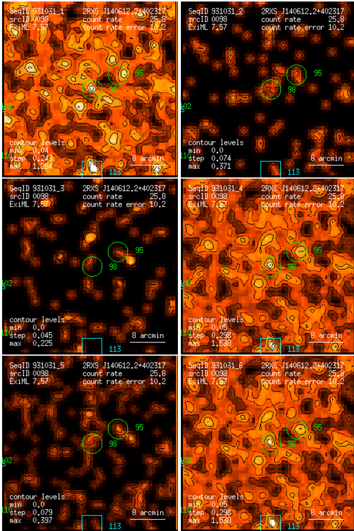
Figure 98: RASS 931031: detection 0098: band rate images, Gaussian filter: (1) PSPC channels 11 – 41, (2) 52 – 90, (3) 91 – 201, (4) 11 – 235, (5) 52 – 201, (6) 11 – 201. Broad band rates in counts/ks. Band rate contour levels in counts/ks/arcmin 2 .
