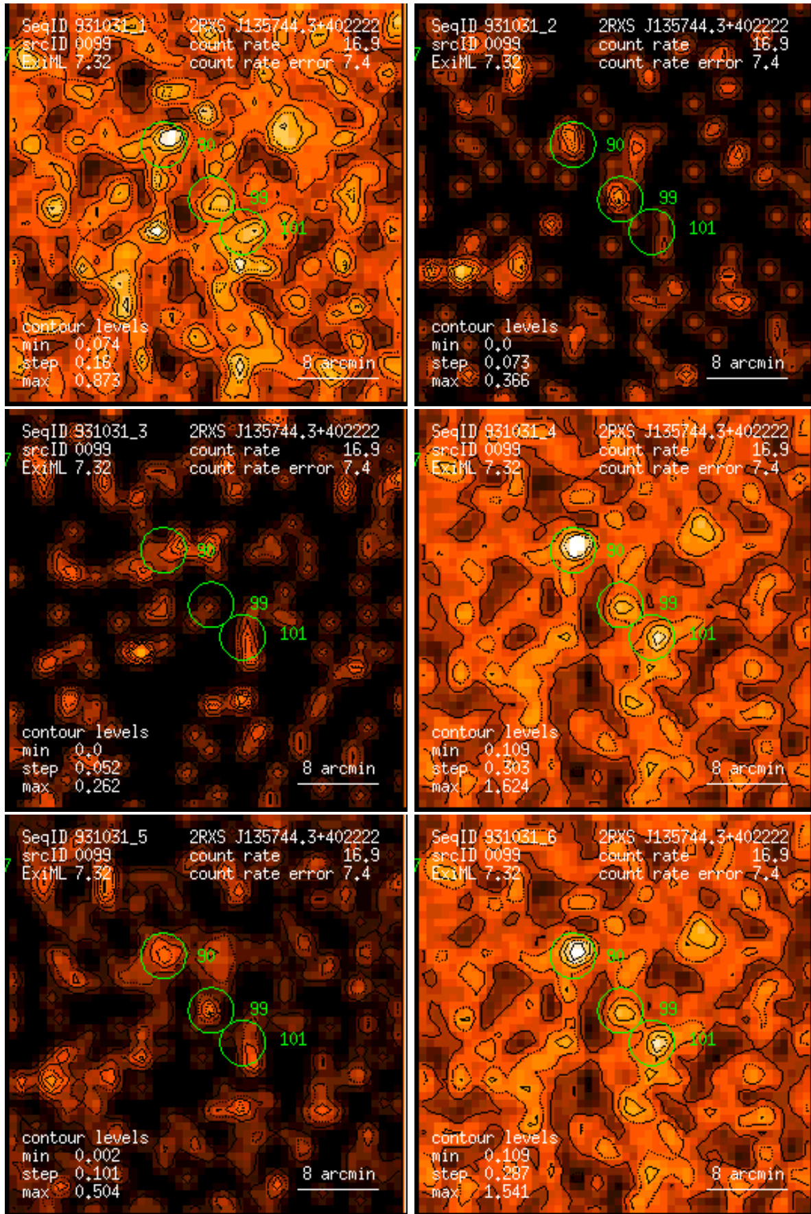
Figure 99: RASS 931031: detection 0099: band rate images, Gaussian filter: (1) PSPC channels 11 – 41, (2) 52 – 90, (3) 91 – 201, (4) 11 – 235, (5) 52 – 201, (6) 11 – 201. Broad band rates in counts/ks. Band rate contour levels in counts/ks/arcmin 2 .
