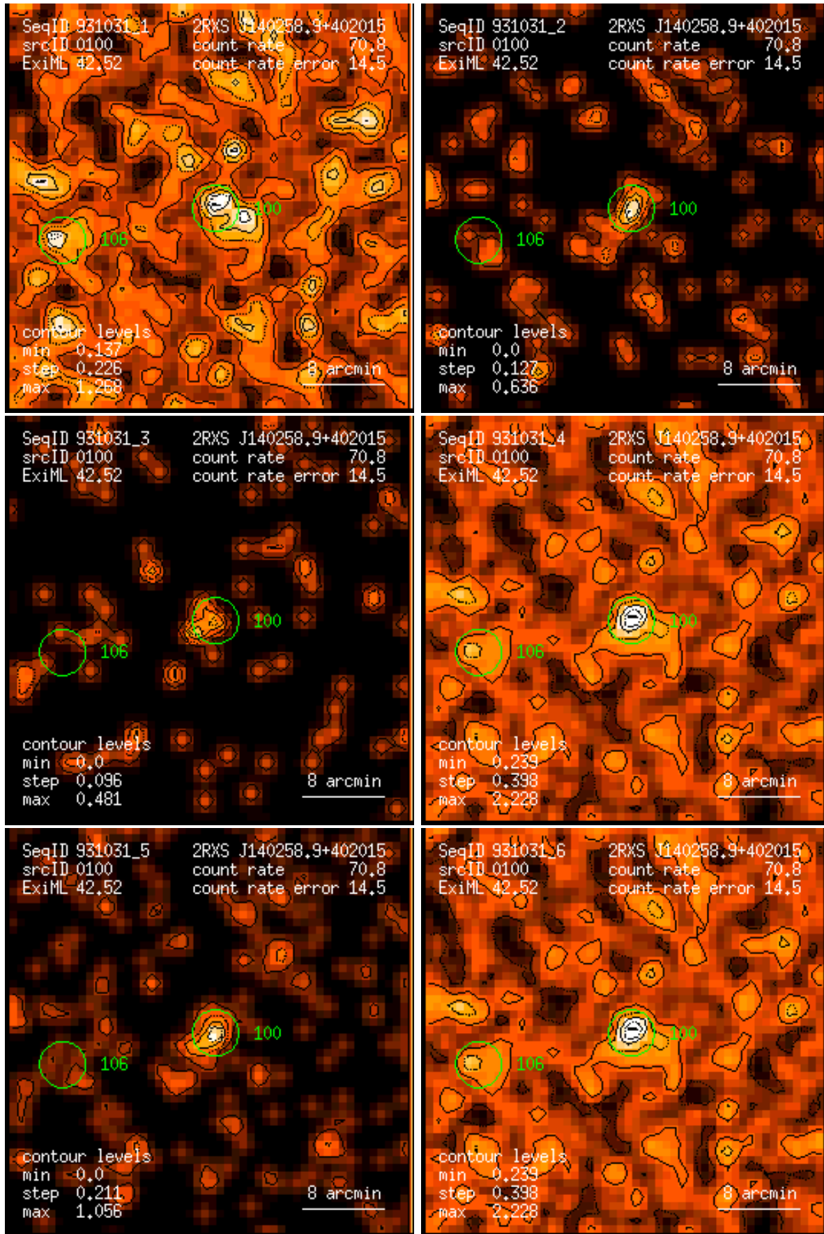
Figure 100: RASS 931031: detection 0100: band rate images, Gaussian filter: (1) PSPC channels 11 – 41, (2) 52 – 90, (3) 91 – 201, (4) 11 – 235, (5) 52 – 201, (6) 11 – 201. Broad band rates in counts/ks. Band rate contour levels in counts/ks/arcmin 2 .
