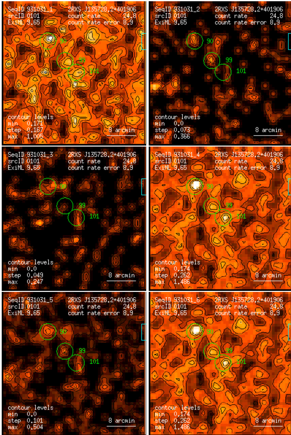
Figure 101: RASS 931031: detection 0101: band rate images, Gaussian filter: (1) PSPC channels 11 – 41, (2) 52 – 90, (3) 91 – 201, (4) 11 – 235, (5) 52 – 201, (6) 11 – 201. Broad band rates in counts/ks. Band rate contour levels in counts/ks/arcmin 2 .
