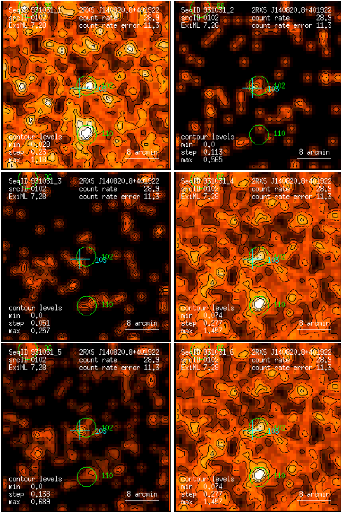
Figure 102: RASS 931031: detection 0102: band rate images, Gaussian filter: (1) PSPC channels 11 – 41, (2) 52 – 90, (3) 91 – 201, (4) 11 – 235, (5) 52 – 201, (6) 11 – 201. Broad band rates in counts/ks. Band rate contour levels in counts/ks/arcmin 2 .
