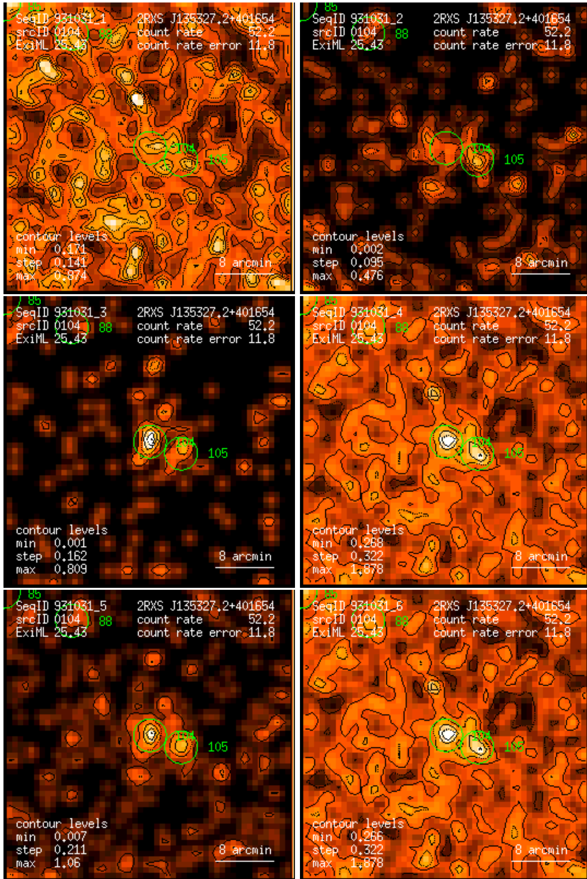
Figure 104: RASS 931031: detection 0104: band rate images, Gaussian filter: (1) PSPC channels 11 – 41, (2) 52 – 90, (3) 91 – 201, (4) 11 – 235, (5) 52 – 201, (6) 11 – 201. Broad band rates in counts/ks. Band rate contour levels in counts/ks/arcmin 2 .
