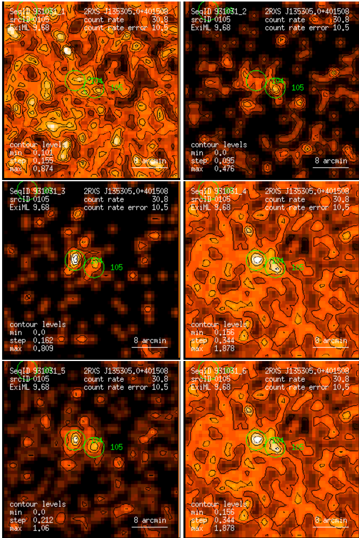
Figure 105: RASS 931031: detection 0105: band rate images, Gaussian filter: (1) PSPC channels 11 – 41, (2) 52 – 90, (3) 91 – 201, (4) 11 – 235, (5) 52 – 201, (6) 11 – 201. Broad band rates in counts/ks. Band rate contour levels in counts/ks/arcmin 2 .
