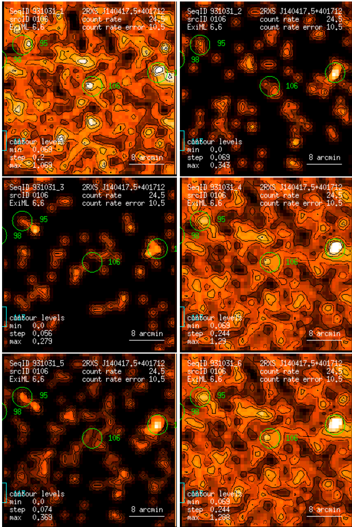
Figure 106: RASS 931031: detection 0106: band rate images, Gaussian filter: (1) PSPC channels 11 – 41, (2) 52 – 90, (3) 91 – 201, (4) 11 – 235, (5) 52 – 201, (6) 11 – 201. Broad band rates in counts/ks. Band rate contour levels in counts/ks/arcmin 2 .
