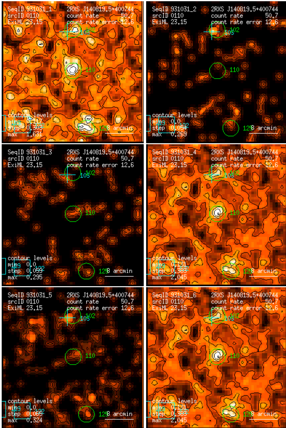
Figure 110: RASS 931031: detection 0110: band rate images, Gaussian filter: (1) PSPC channels 11 – 41, (2) 52 – 90, (3) 91 – 201, (4) 11 – 235, (5) 52 – 201, (6) 11 – 201. Broad band rates in counts/ks. Band rate contour levels in counts/ks/arcmin 2 .
