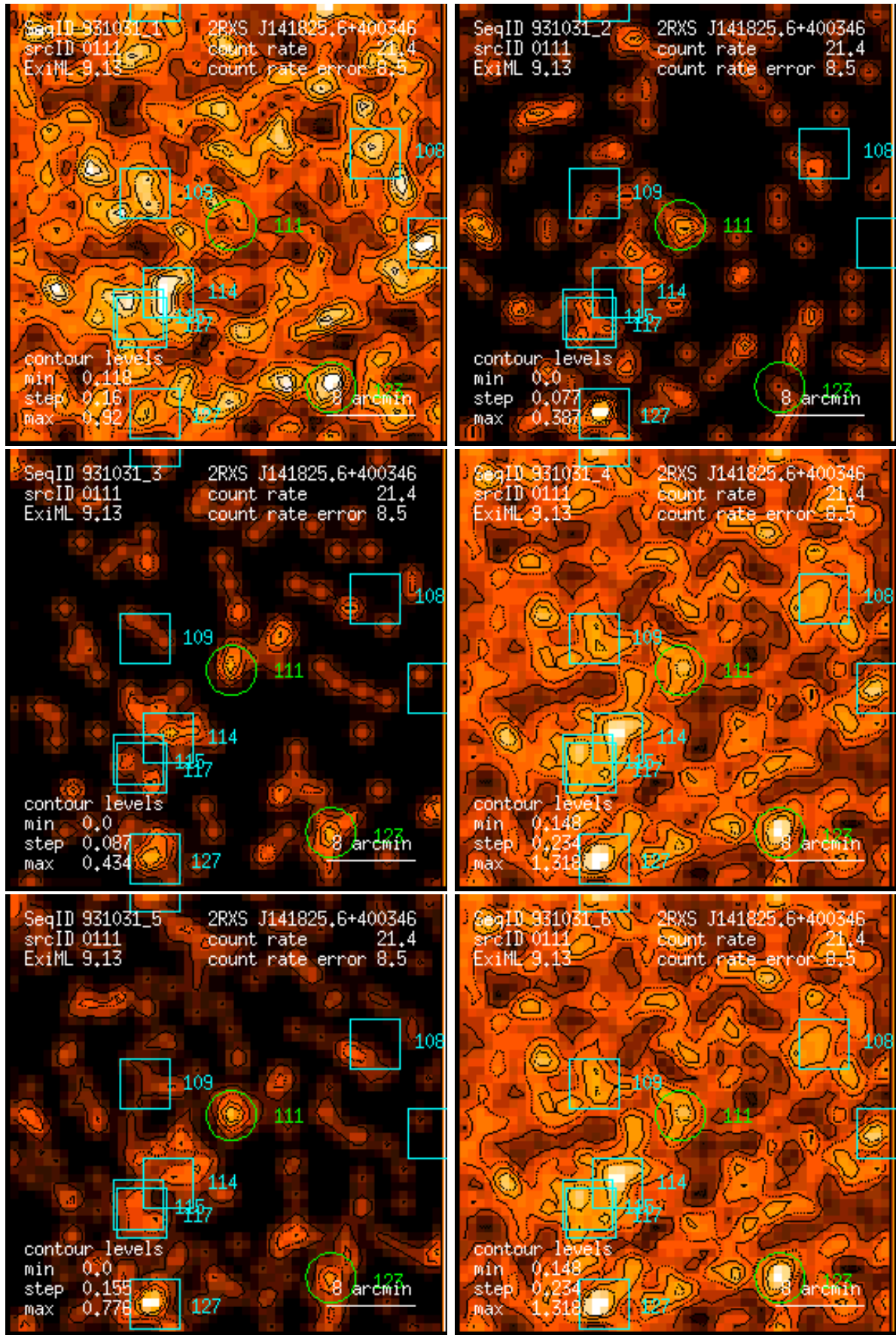
Figure 111: RASS 931031: detection 0111: band rate images, Gaussian filter: (1) PSPC channels 11 – 41, (2) 52 – 90, (3) 91 – 201, (4) 11 – 235, (5) 52 – 201, (6) 11 – 201. Broad band rates in counts/ks. Band rate contour levels in counts/ks/arcmin 2 .
