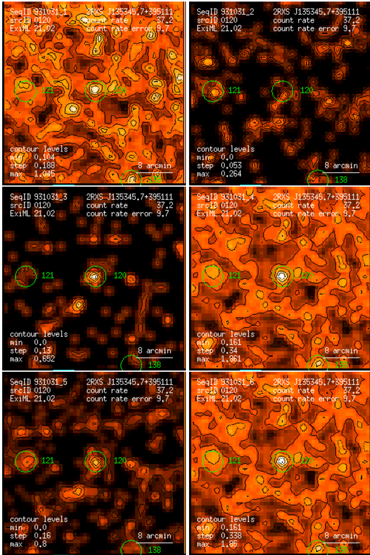
Figure 120: RASS 931031: detection 0120: band rate images, Gaussian filter: (1) PSPC channels 11 – 41, (2) 52 – 90, (3) 91 – 201, (4) 11 – 235, (5) 52 – 201, (6) 11 – 201. Broad band rates in counts/ks. Band rate contour levels in counts/ks/arcmin 2 .
