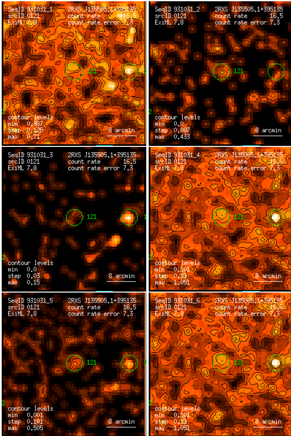
Figure 121: RASS 931031: detection 0121: band rate images, Gaussian filter: (1) PSPC channels 11 – 41, (2) 52 – 90, (3) 91 – 201, (4) 11 – 235, (5) 52 – 201, (6) 11 – 201. Broad band rates in counts/ks. Band rate contour levels in counts/ks/arcmin 2 .
