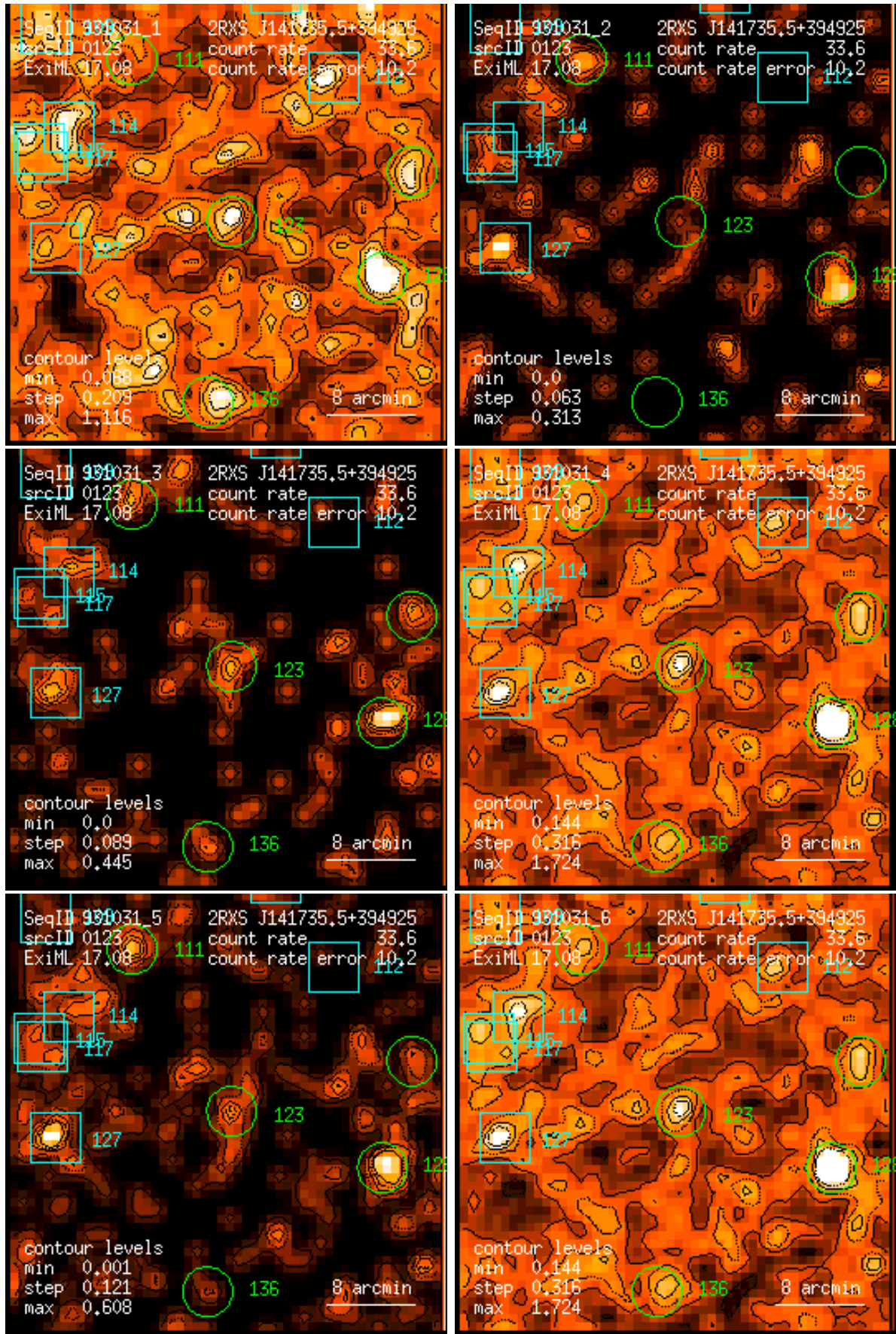
Figure 123: RASS 931031: detection 0123: band rate images, Gaussian filter: (1) PSPC channels 11 – 41, (2) 52 – 90, (3) 91 – 201, (4) 11 – 235, (5) 52 – 201, (6) 11 – 201. Broad band rates in counts/ks. Band rate contour levels in counts/ks/arcmin 2 .
