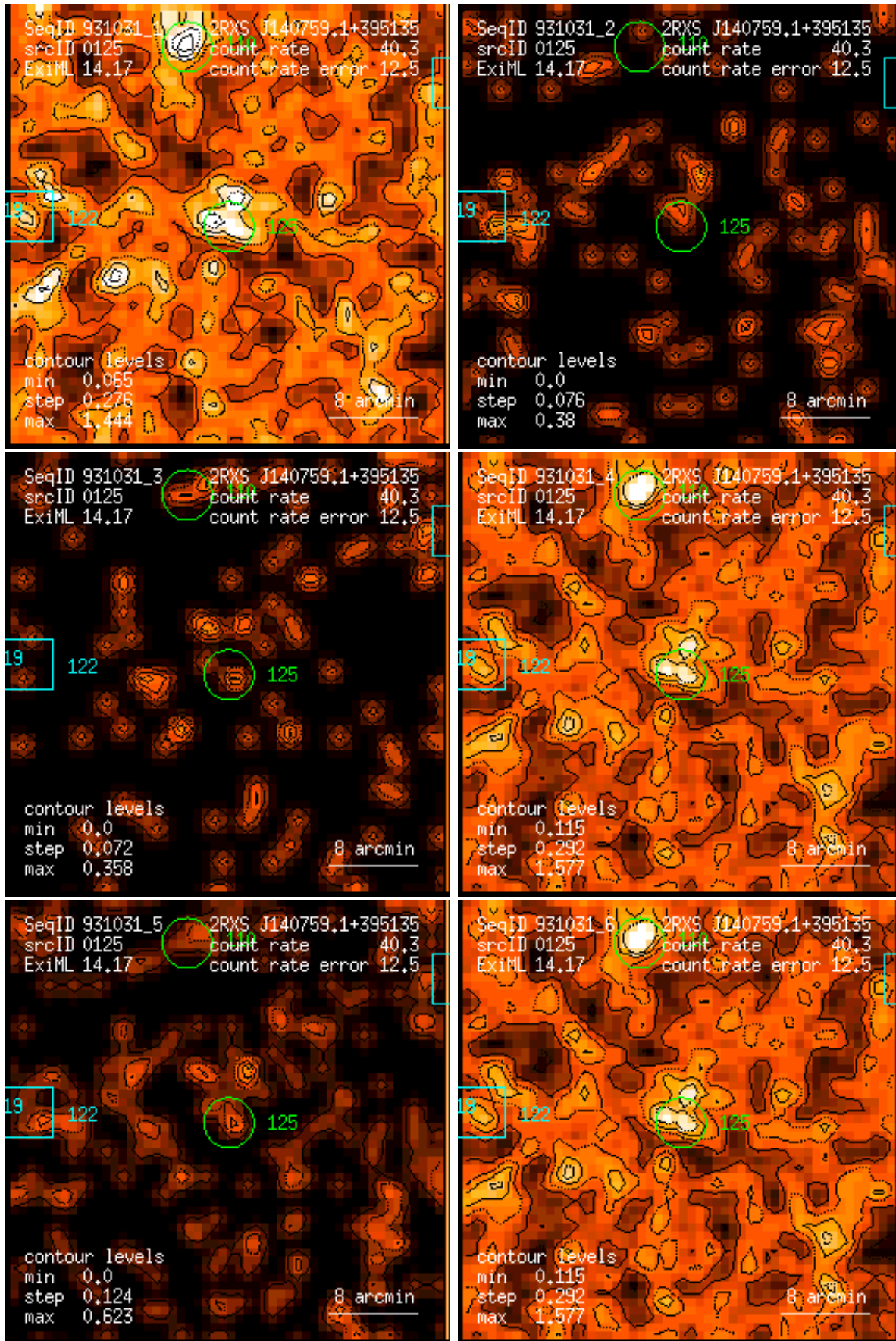
Figure 125: RASS 931031: detection 0125: band rate images, Gaussian filter: (1) PSPC channels 11 – 41, (2) 52 – 90, (3) 91 – 201, (4) 11 – 235, (5) 52 – 201, (6) 11 – 201. Broad band rates in counts/ks. Band rate contour levels in counts/ks/arcmin 2 .
