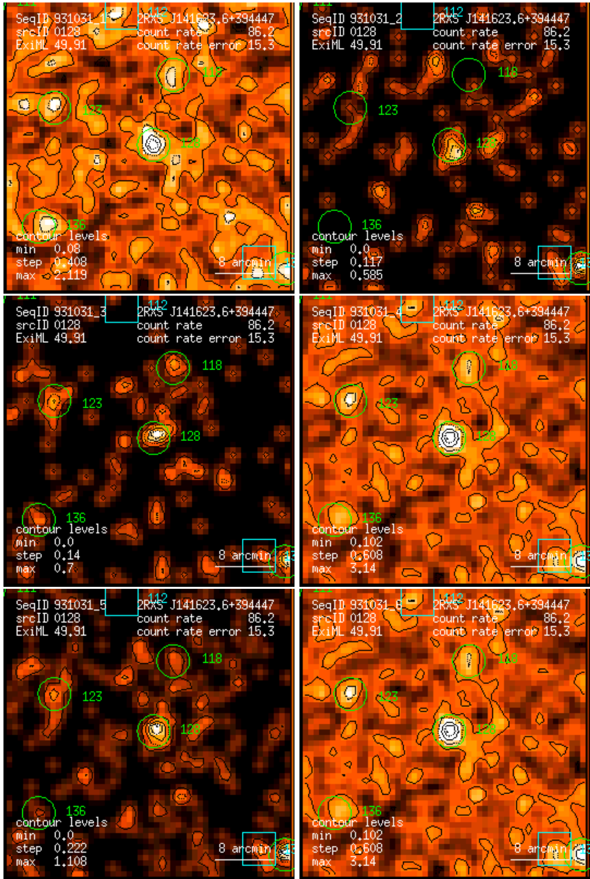
Figure 128: RASS 931031: detection 0128: band rate images, Gaussian filter: (1) PSPC channels 11 – 41, (2) 52 – 90, (3) 91 – 201, (4) 11 – 235, (5) 52 – 201, (6) 11 – 201. Broad band rates in counts/ks. Band rate contour levels in counts/ks/arcmin 2 .
