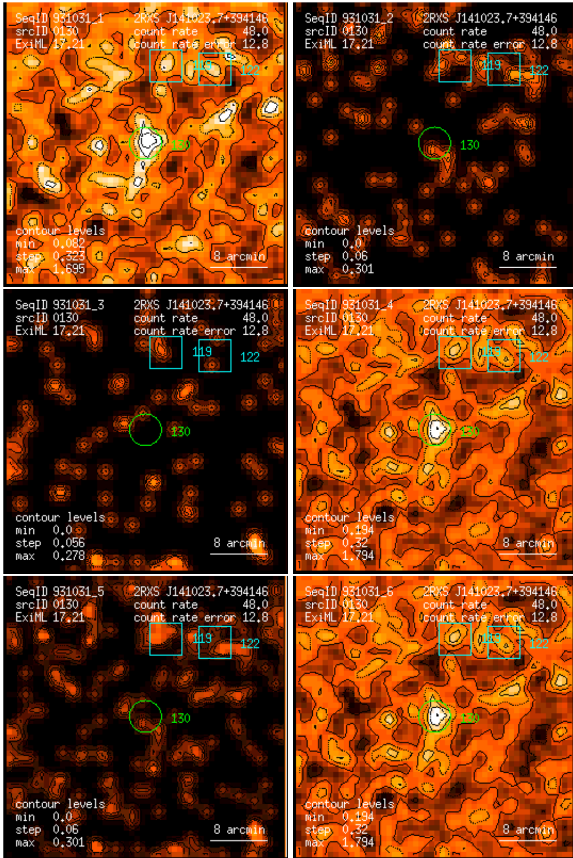
Figure 130: RASS 931031: detection 0130: band rate images, Gaussian filter: (1) PSPC channels 11 – 41, (2) 52 – 90, (3) 91 – 201, (4) 11 – 235, (5) 52 – 201, (6) 11 – 201. Broad band rates in counts/ks. Band rate contour levels in counts/ks/arcmin 2 .
