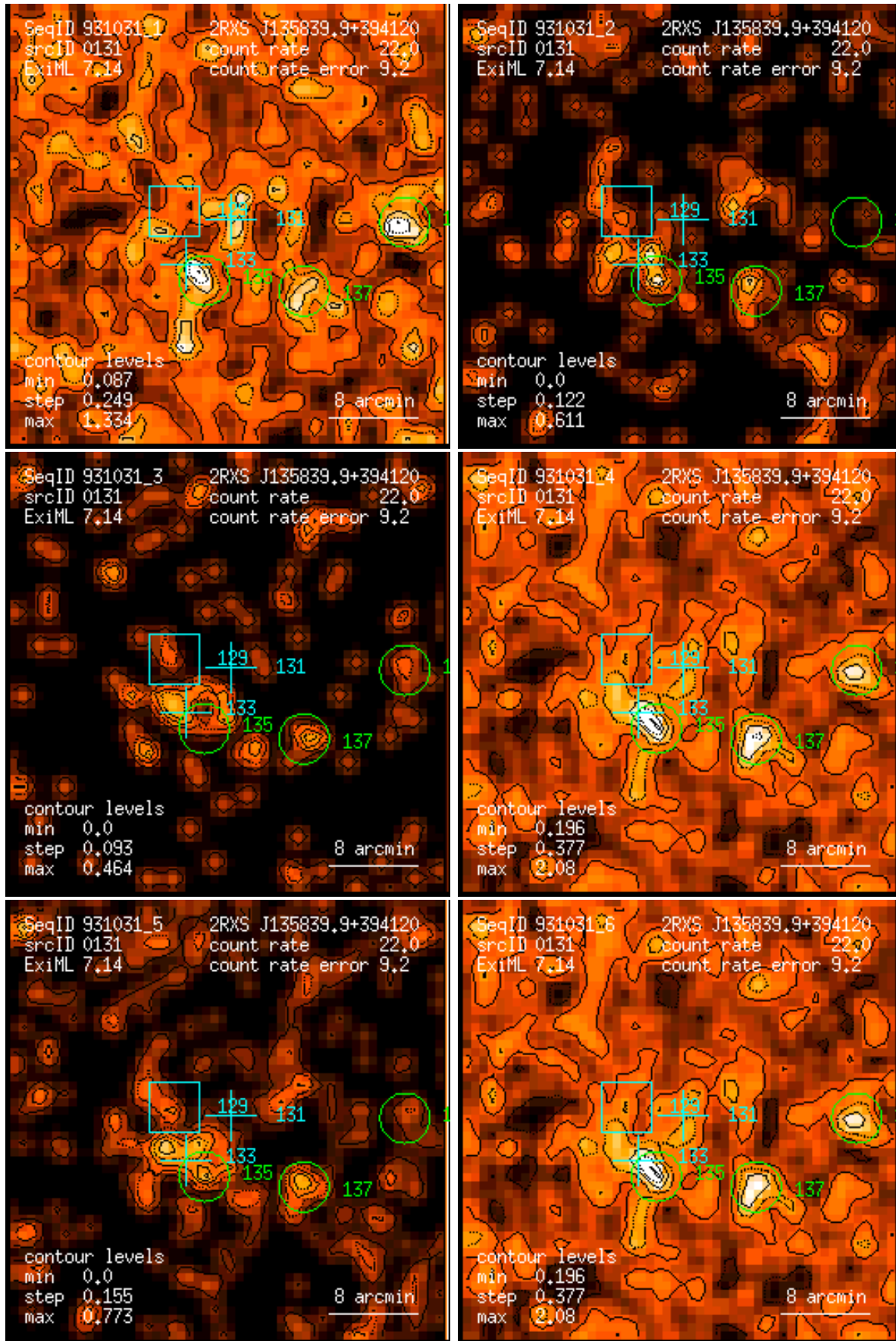
Figure 131: RASS 931031: detection 0131: band rate images, Gaussian filter: (1) PSPC channels 11 – 41, (2) 52 – 90, (3) 91 – 201, (4) 11 – 235, (5) 52 – 201, (6) 11 – 201. Broad band rates in counts/ks. Band rate contour levels in counts/ks/arcmin 2 .
