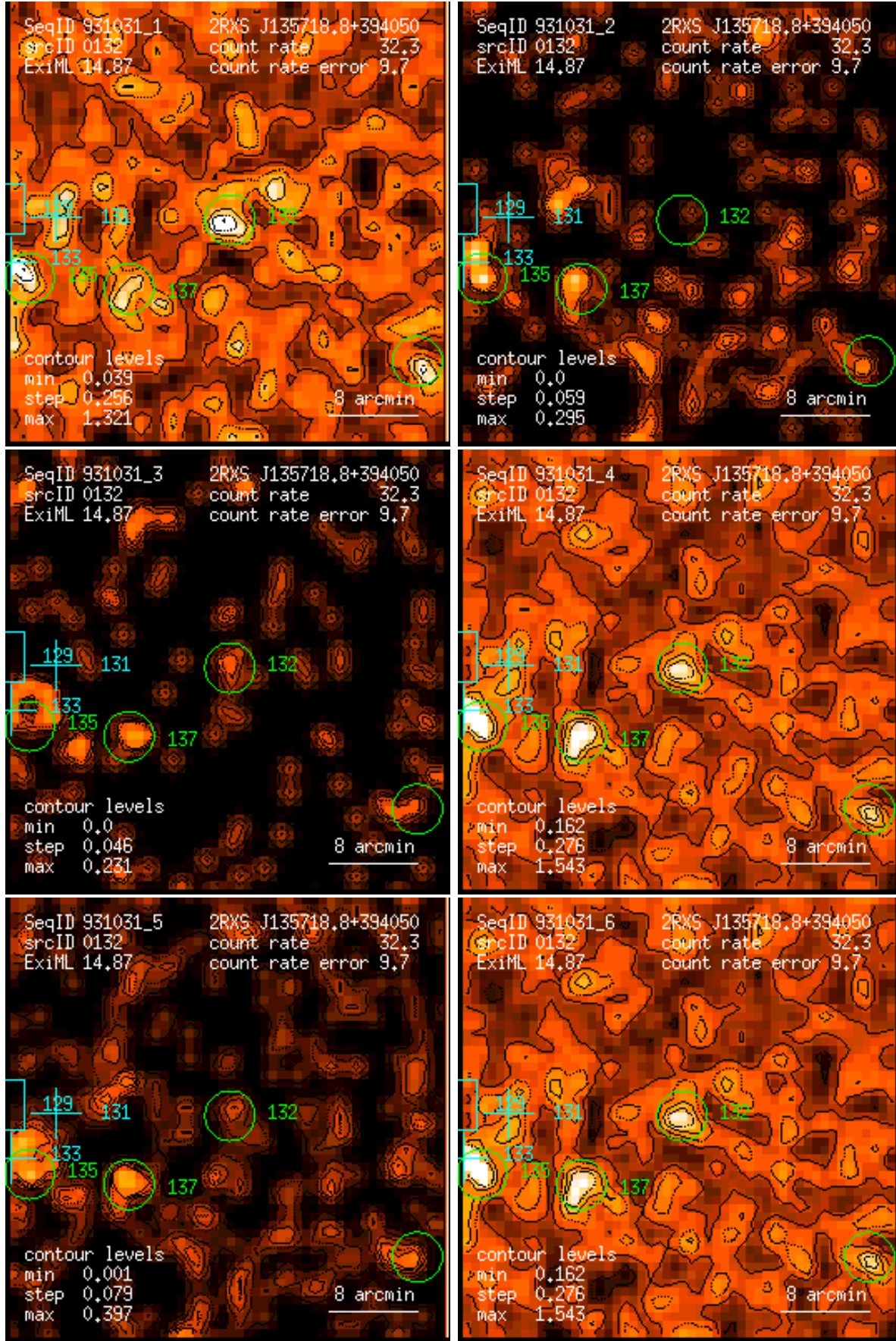
Figure 132: RASS 931031: detection 0132: band rate images, Gaussian filter: (1) PSPC channels 11 – 41, (2) 52 – 90, (3) 91 – 201, (4) 11 – 235, (5) 52 – 201, (6) 11 – 201. Broad band rates in counts/ks. Band rate contour levels in counts/ks/arcmin 2 .
