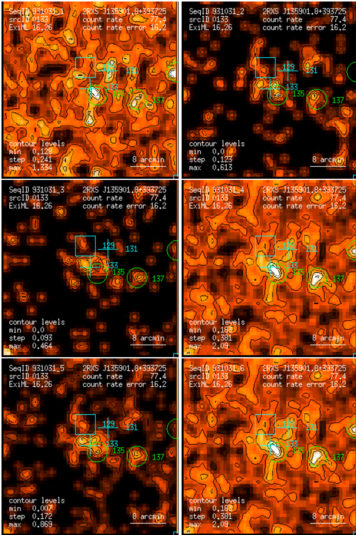
Figure 133: RASS 931031: detection 0133: band rate images, Gaussian filter: (1) PSPC channels 11 – 41, (2) 52 – 90, (3) 91 – 201, (4) 11 – 235, (5) 52 – 201, (6) 11 – 201. Broad band rates in counts/ks. Band rate contour levels in counts/ks/arcmin 2 .
