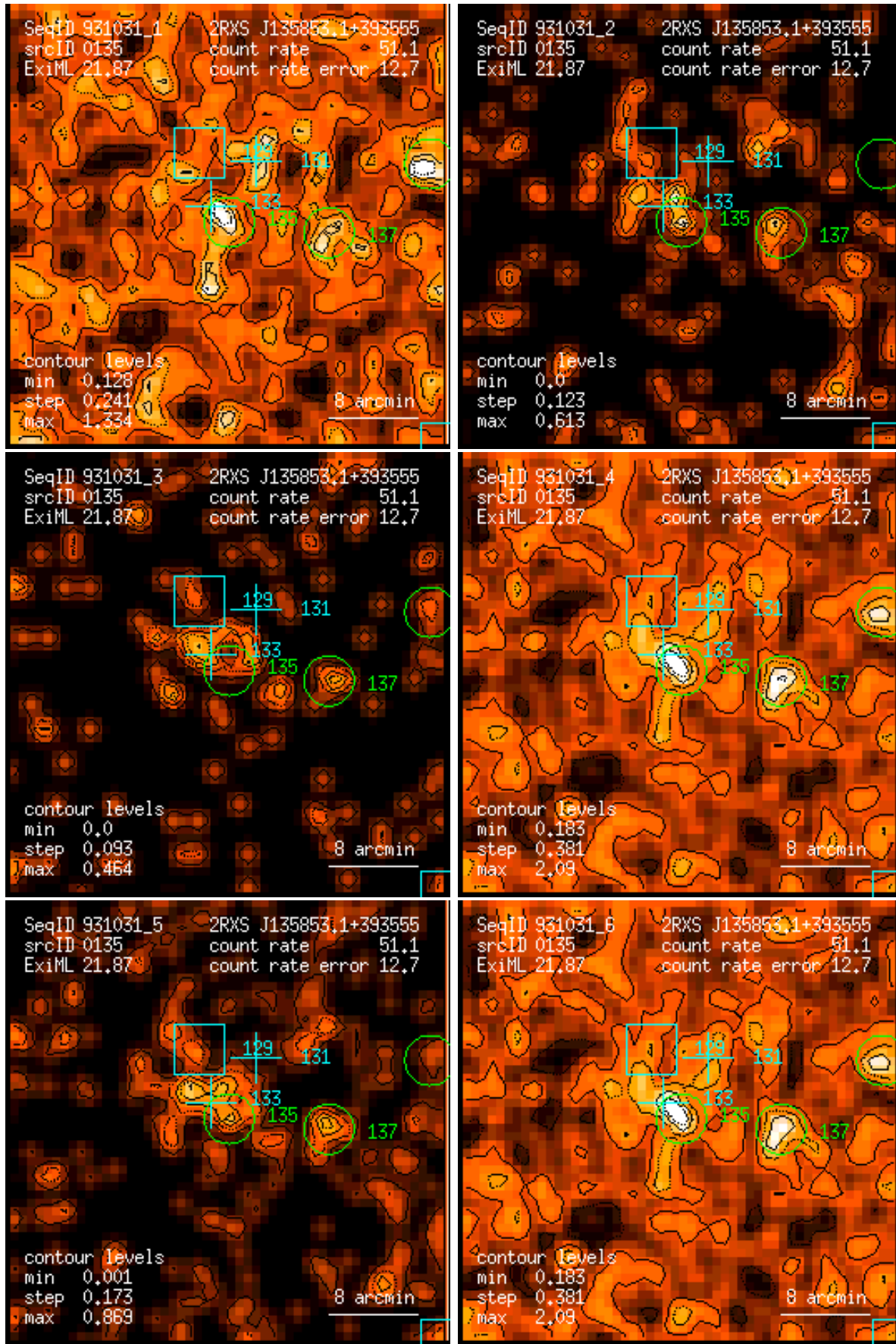
Figure 135: RASS 931031: detection 0135: band rate images, Gaussian filter: (1) PSPC channels 11 – 41, (2) 52 – 90, (3) 91 – 201, (4) 11 – 235, (5) 52 – 201, (6) 11 – 201. Broad band rates in counts/ks. Band rate contour levels in counts/ks/arcmin 2 .
