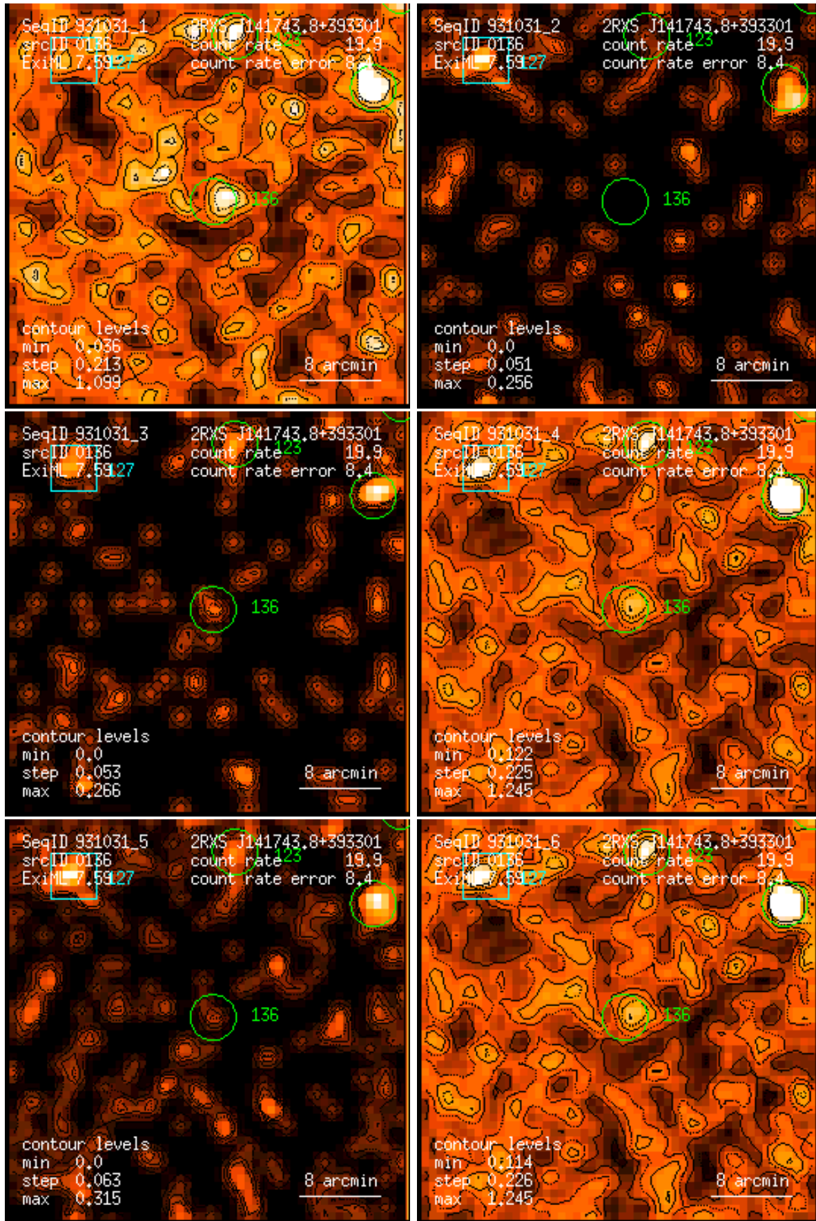
Figure 136: RASS 931031: detection 0136: band rate images, Gaussian filter: (1) PSPC channels 11 – 41, (2) 52 – 90, (3) 91 – 201, (4) 11 – 235, (5) 52 – 201, (6) 11 – 201. Broad band rates in counts/ks. Band rate contour levels in counts/ks/arcmin 2 .
