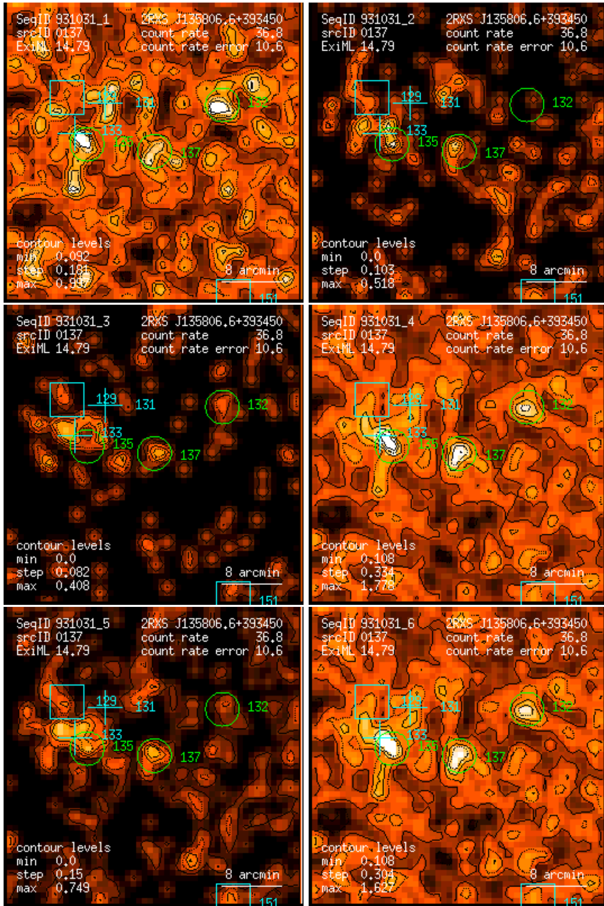
Figure 137: RASS 931031: detection 0137: band rate images, Gaussian filter: (1) PSPC channels 11 – 41, (2) 52 – 90, (3) 91 – 201, (4) 11 – 235, (5) 52 – 201, (6) 11 – 201. Broad band rates in counts/ks. Band rate contour levels in counts/ks/arcmin 2 .
