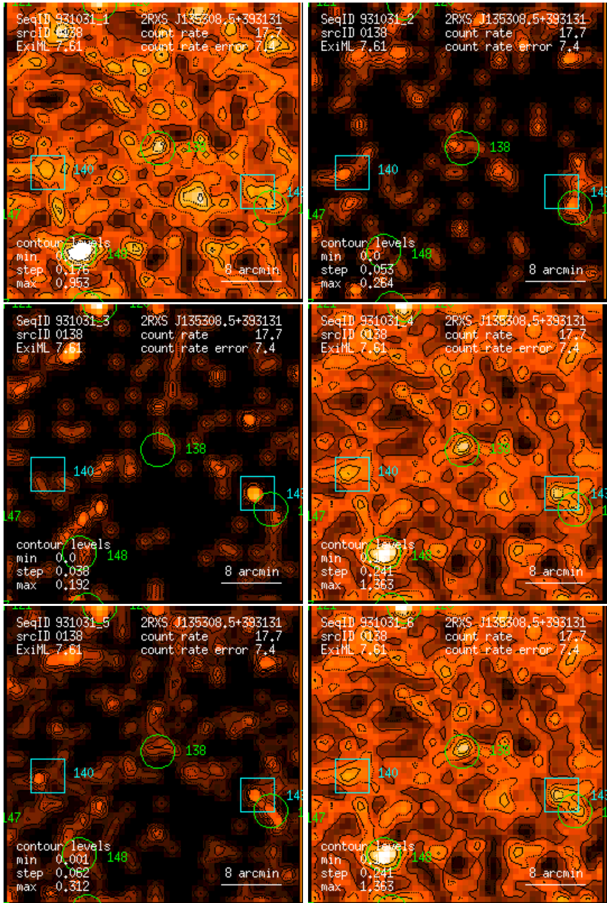
Figure 138: RASS 931031: detection 0138: band rate images, Gaussian filter: (1) PSPC channels 11 – 41, (2) 52 – 90, (3) 91 – 201, (4) 11 – 235, (5) 52 – 201, (6) 11 – 201. Broad band rates in counts/ks. Band rate contour levels in counts/ks/arcmin 2 .
