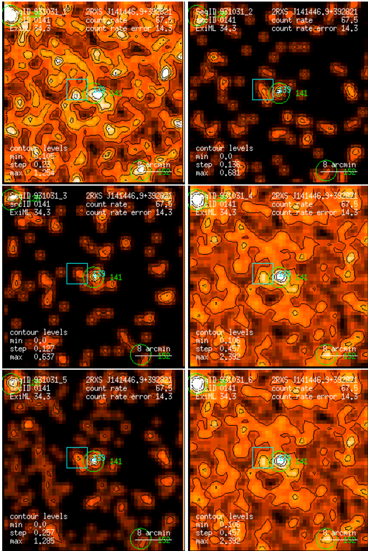
Figure 141: RASS 931031: detection 0141: band rate images, Gaussian filter: (1) PSPC channels 11 – 41, (2) 52 – 90, (3) 91 – 201, (4) 11 – 235, (5) 52 – 201, (6) 11 – 201. Broad band rates in counts/ks. Band rate contour levels in counts/ks/arcmin 2 .
