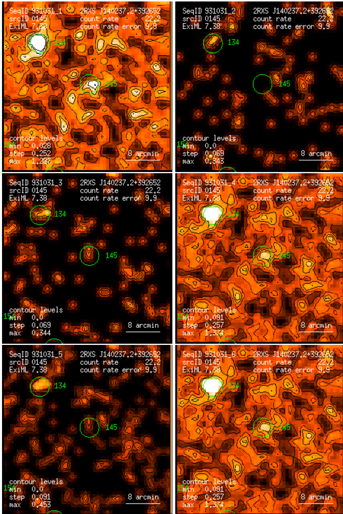
Figure 145: RASS 931031: detection 0145: band rate images, Gaussian filter: (1) PSPC channels 11 – 41, (2) 52 – 90, (3) 91 – 201, (4) 11 – 235, (5) 52 – 201, (6) 11 – 201. Broad band rates in counts/ks. Band rate contour levels in counts/ks/arcmin 2 .
