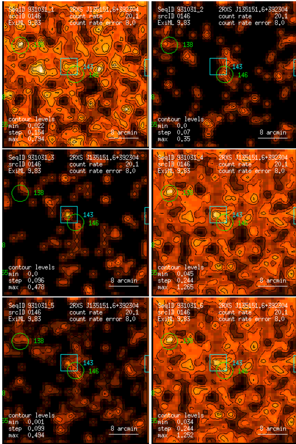
Figure 146: RASS 931031: detection 0146: band rate images, Gaussian filter: (1) PSPC channels 11 – 41, (2) 52 – 90, (3) 91 – 201, (4) 11 – 235, (5) 52 – 201, (6) 11 – 201. Broad band rates in counts/ks. Band rate contour levels in counts/ks/arcmin 2 .
