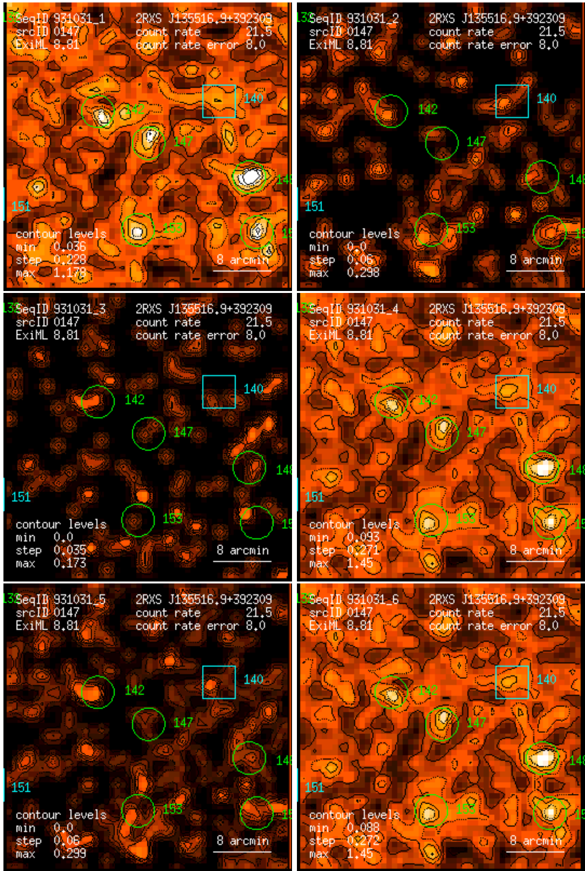
Figure 147: RASS 931031: detection 0147: band rate images, Gaussian filter: (1) PSPC channels 11 – 41, (2) 52 – 90, (3) 91 – 201, (4) 11 – 235, (5) 52 – 201, (6) 11 – 201. Broad band rates in counts/ks. Band rate contour levels in counts/ks/arcmin 2 .
