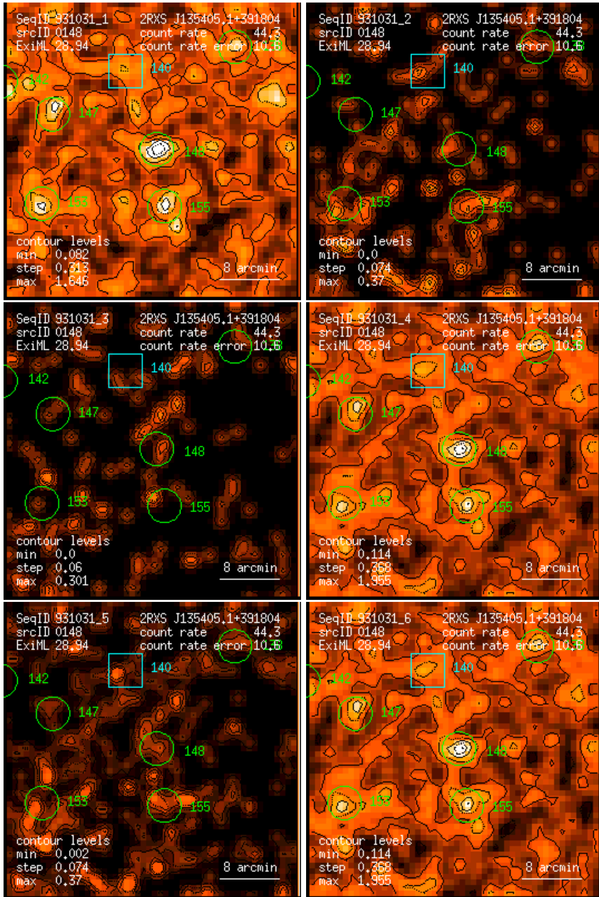
Figure 148: RASS 931031: detection 0148: band rate images, Gaussian filter: (1) PSPC channels 11 – 41, (2) 52 – 90, (3) 91 – 201, (4) 11 – 235, (5) 52 – 201, (6) 11 – 201. Broad band rates in counts/ks. Band rate contour levels in counts/ks/arcmin 2 .
