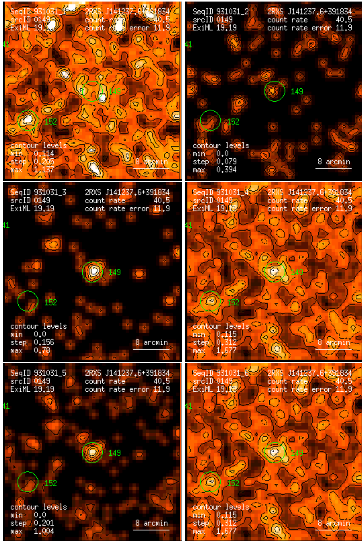
Figure 149: RASS 931031: detection 0149: band rate images, Gaussian filter: (1) PSPC channels 11 – 41, (2) 52 – 90, (3) 91 – 201, (4) 11 – 235, (5) 52 – 201, (6) 11 – 201. Broad band rates in counts/ks. Band rate contour levels in counts/ks/arcmin 2 .
