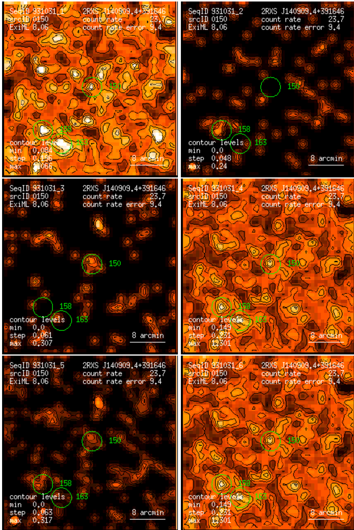
Figure 150: RASS 931031: detection 0150: band rate images, Gaussian filter: (1) PSPC channels 11 – 41, (2) 52 – 90, (3) 91 – 201, (4) 11 – 235, (5) 52 – 201, (6) 11 – 201. Broad band rates in counts/ks. Band rate contour levels in counts/ks/arcmin 2 .
