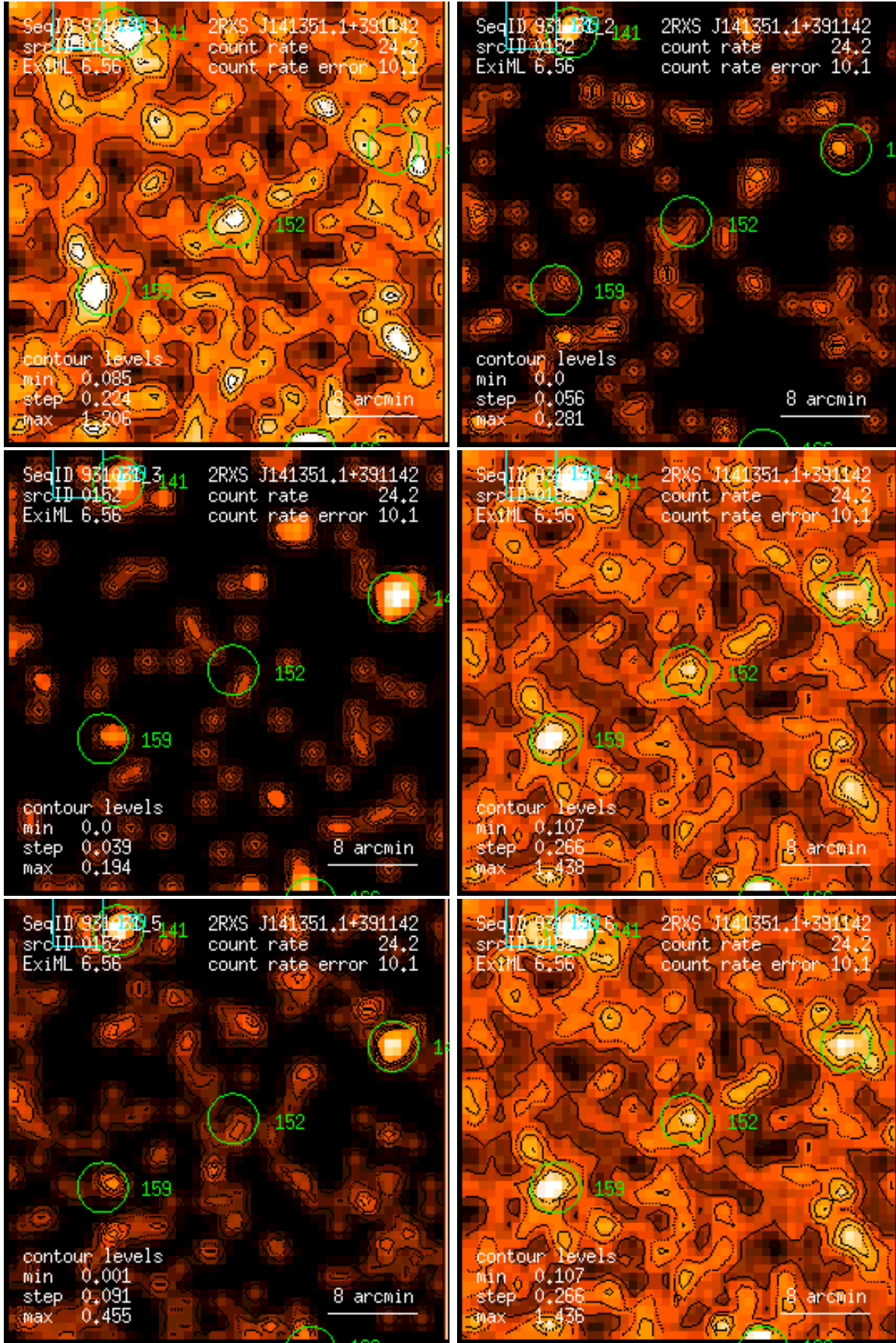
Figure 152: RASS 931031: detection 0152: band rate images, Gaussian filter: (1) PSPC channels 11 – 41, (2) 52 – 90, (3) 91 – 201, (4) 11 – 235, (5) 52 – 201, (6) 11 – 201. Broad band rates in counts/ks. Band rate contour levels in counts/ks/arcmin 2 .
