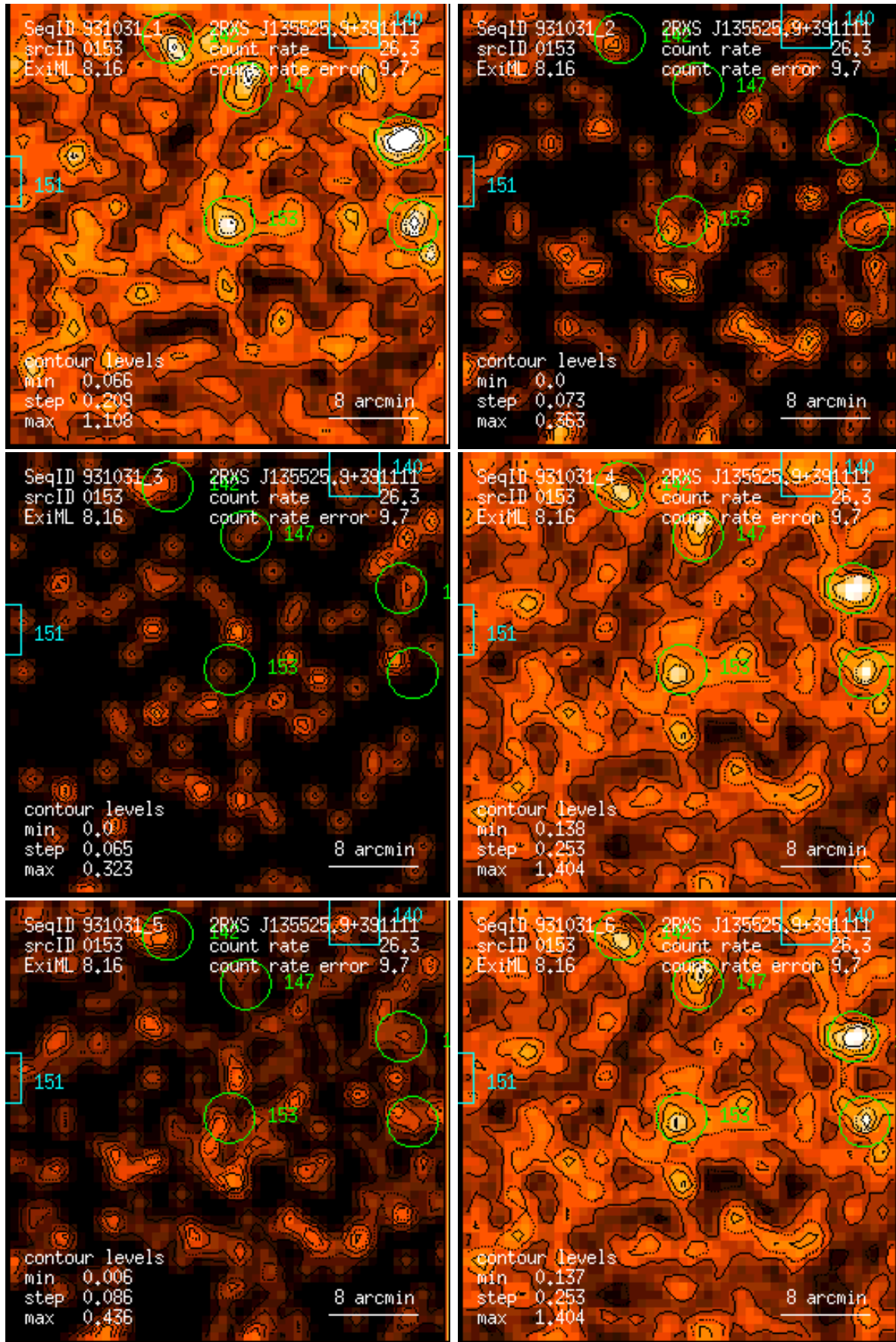
Figure 153: RASS 931031: detection 0153: band rate images, Gaussian filter: (1) PSPC channels 11 – 41, (2) 52 – 90, (3) 91 – 201, (4) 11 – 235, (5) 52 – 201, (6) 11 – 201. Broad band rates in counts/ks. Band rate contour levels in counts/ks/arcmin 2 .
