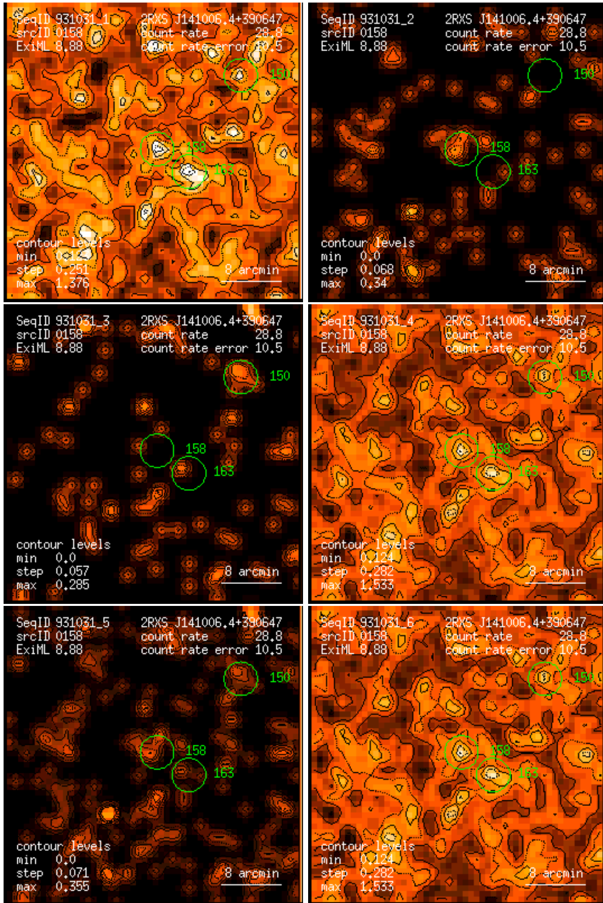
Figure 158: RASS 931031: detection 0158: band rate images, Gaussian filter: (1) PSPC channels 11 – 41, (2) 52 – 90, (3) 91 – 201, (4) 11 – 235, (5) 52 – 201, (6) 11 – 201. Broad band rates in counts/ks. Band rate contour levels in counts/ks/arcmin 2 .
