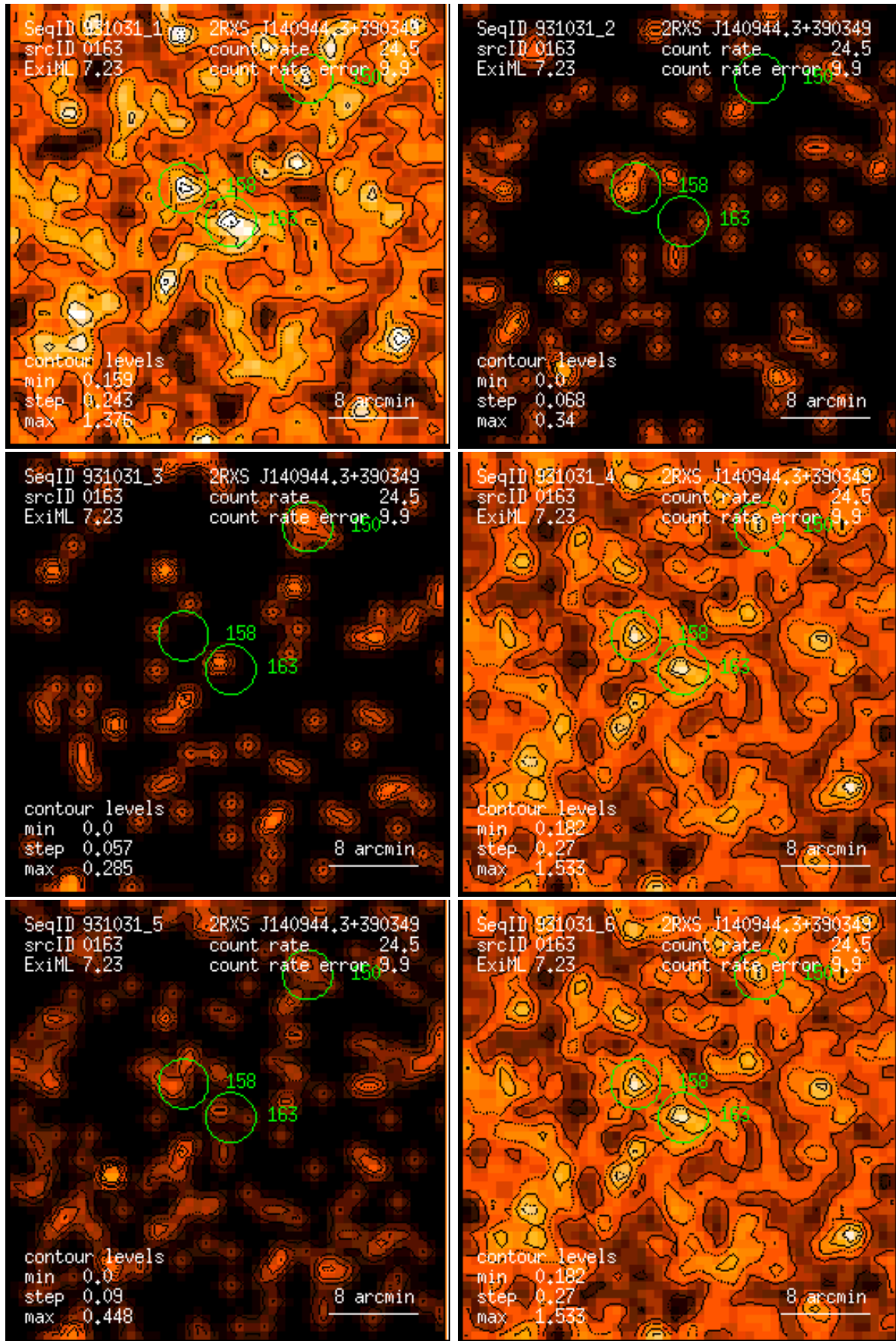
Figure 163: RASS 931031: detection 0163: band rate images, Gaussian filter: (1) PSPC channels 11 – 41, (2) 52 – 90, (3) 91 – 201, (4) 11 – 235, (5) 52 – 201, (6) 11 – 201. Broad band rates in counts/ks. Band rate contour levels in counts/ks/arcmin 2 .
