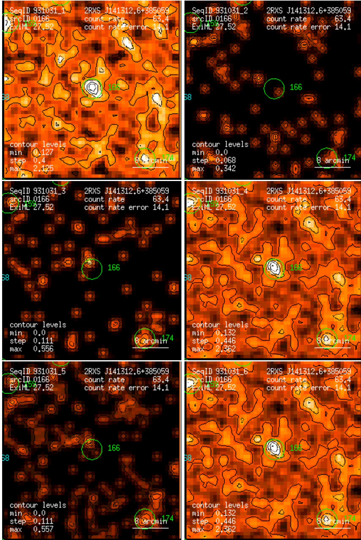
Figure 166: RASS 931031: detection 0166: band rate images, Gaussian filter: (1) PSPC channels 11 – 41, (2) 52 – 90, (3) 91 – 201, (4) 11 – 235, (5) 52 – 201, (6) 11 – 201. Broad band rates in counts/ks. Band rate contour levels in counts/ks/arcmin 2 .
