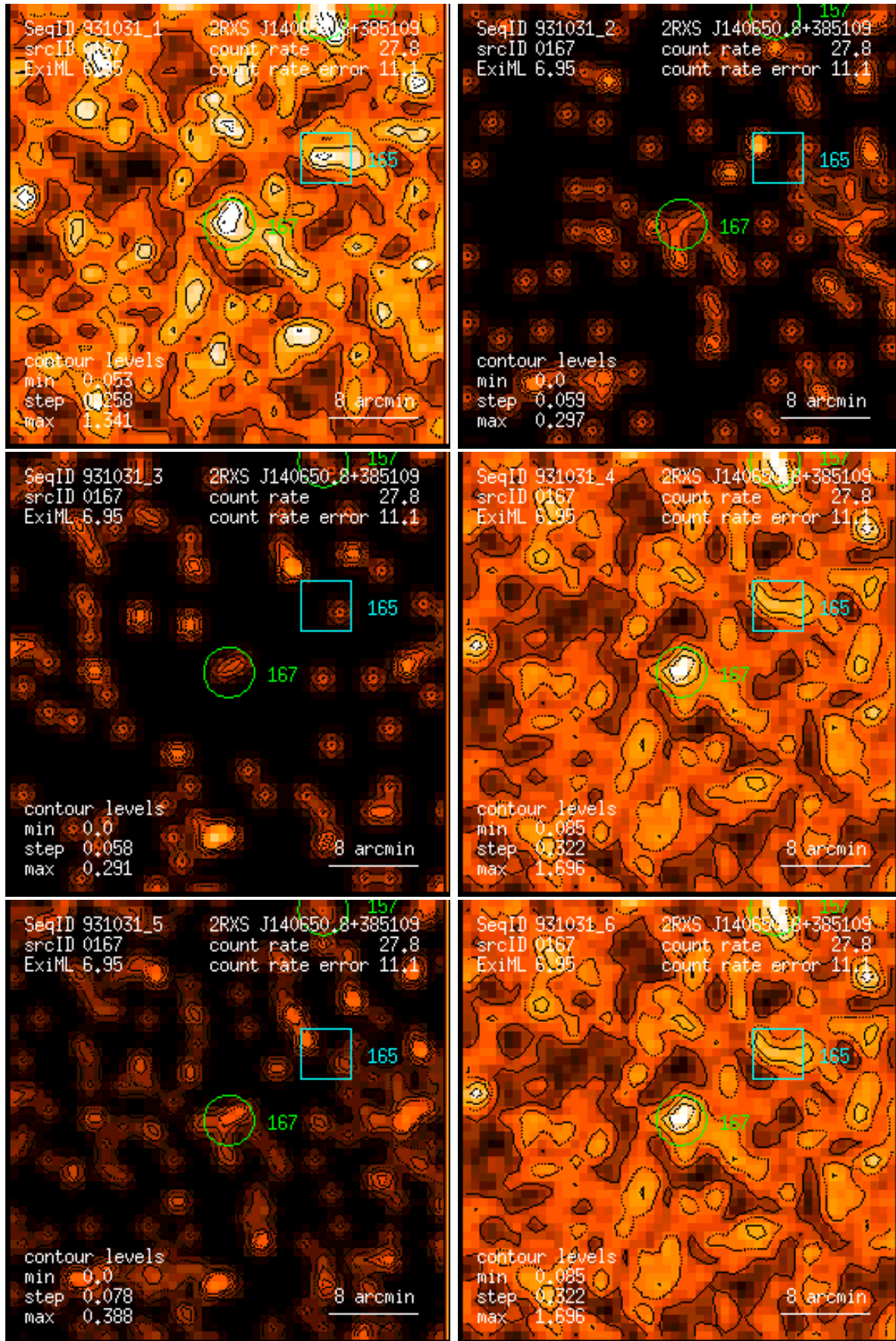
Figure 167: RASS 931031: detection 0167: band rate images, Gaussian filter: (1) PSPC channels 11 – 41, (2) 52 – 90, (3) 91 – 201, (4) 11 – 235, (5) 52 – 201, (6) 11 – 201. Broad band rates in counts/ks. Band rate contour levels in counts/ks/arcmin 2 .
