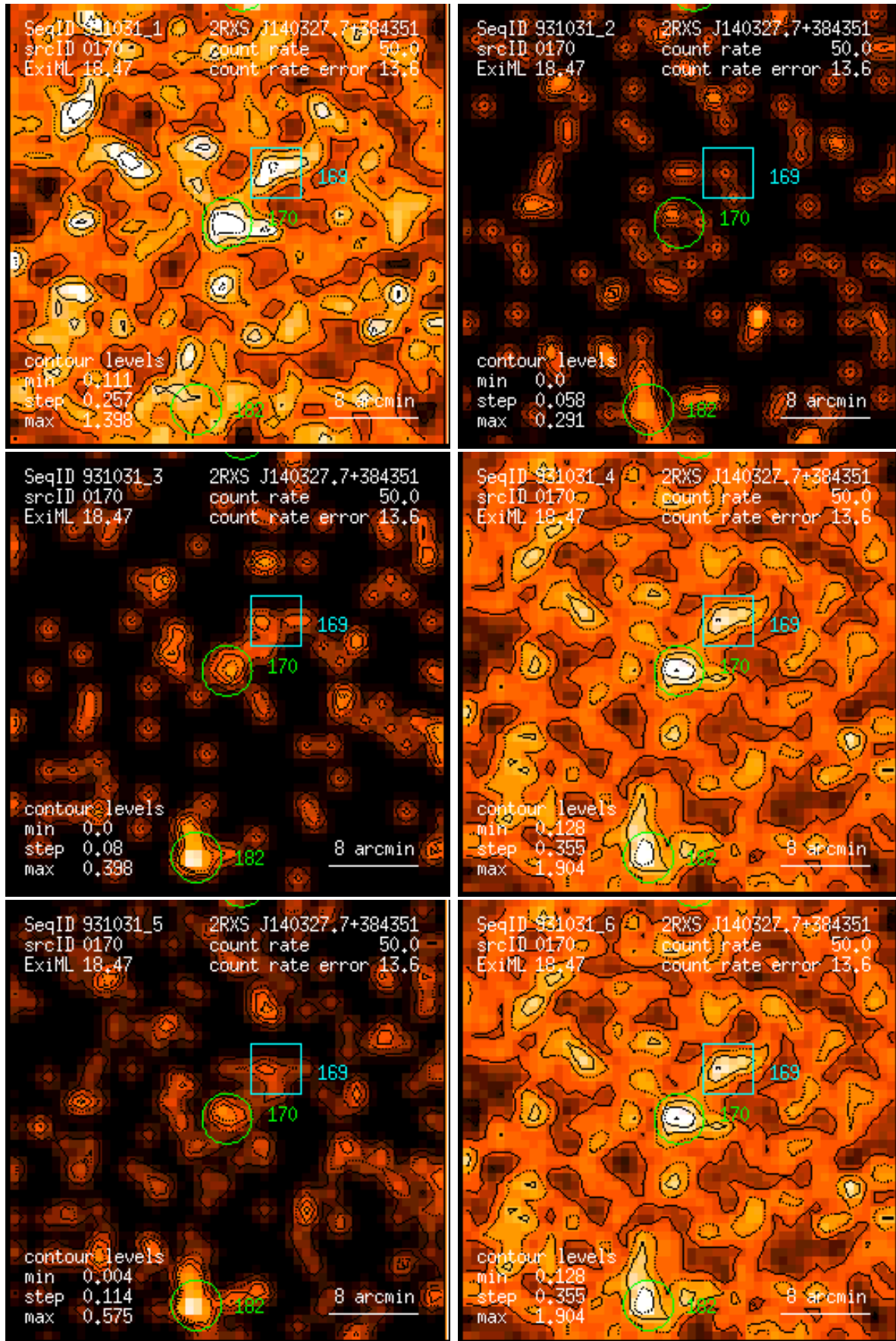
Figure 170: RASS 931031: detection 0170: band rate images, Gaussian filter: (1) PSPC channels 11 – 41, (2) 52 – 90, (3) 91 – 201, (4) 11 – 235, (5) 52 – 201, (6) 11 – 201. Broad band rates in counts/ks. Band rate contour levels in counts/ks/arcmin 2 .
