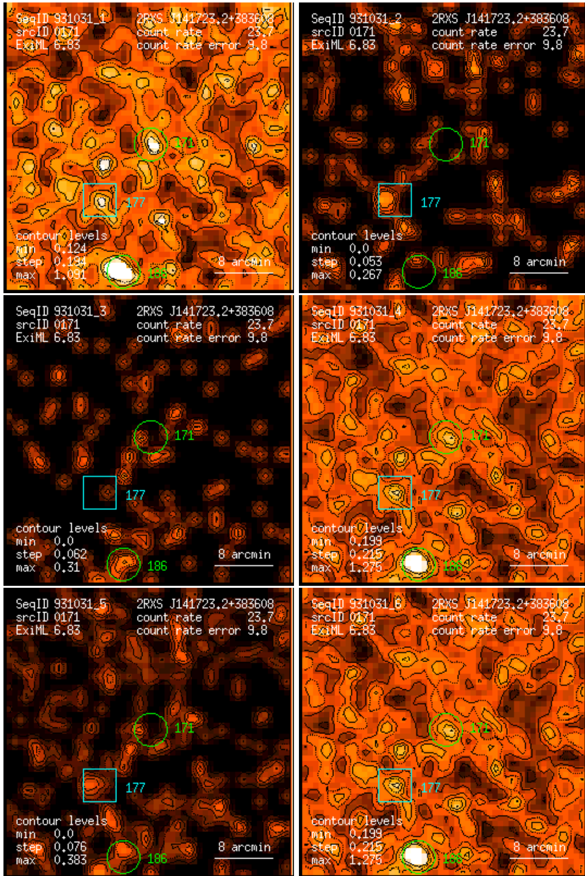
Figure 171: RASS 931031: detection 0171: band rate images, Gaussian filter: (1) PSPC channels 11 – 41, (2) 52 – 90, (3) 91 – 201, (4) 11 – 235, (5) 52 – 201, (6) 11 – 201. Broad band rates in counts/ks. Band rate contour levels in counts/ks/arcmin 2 .
