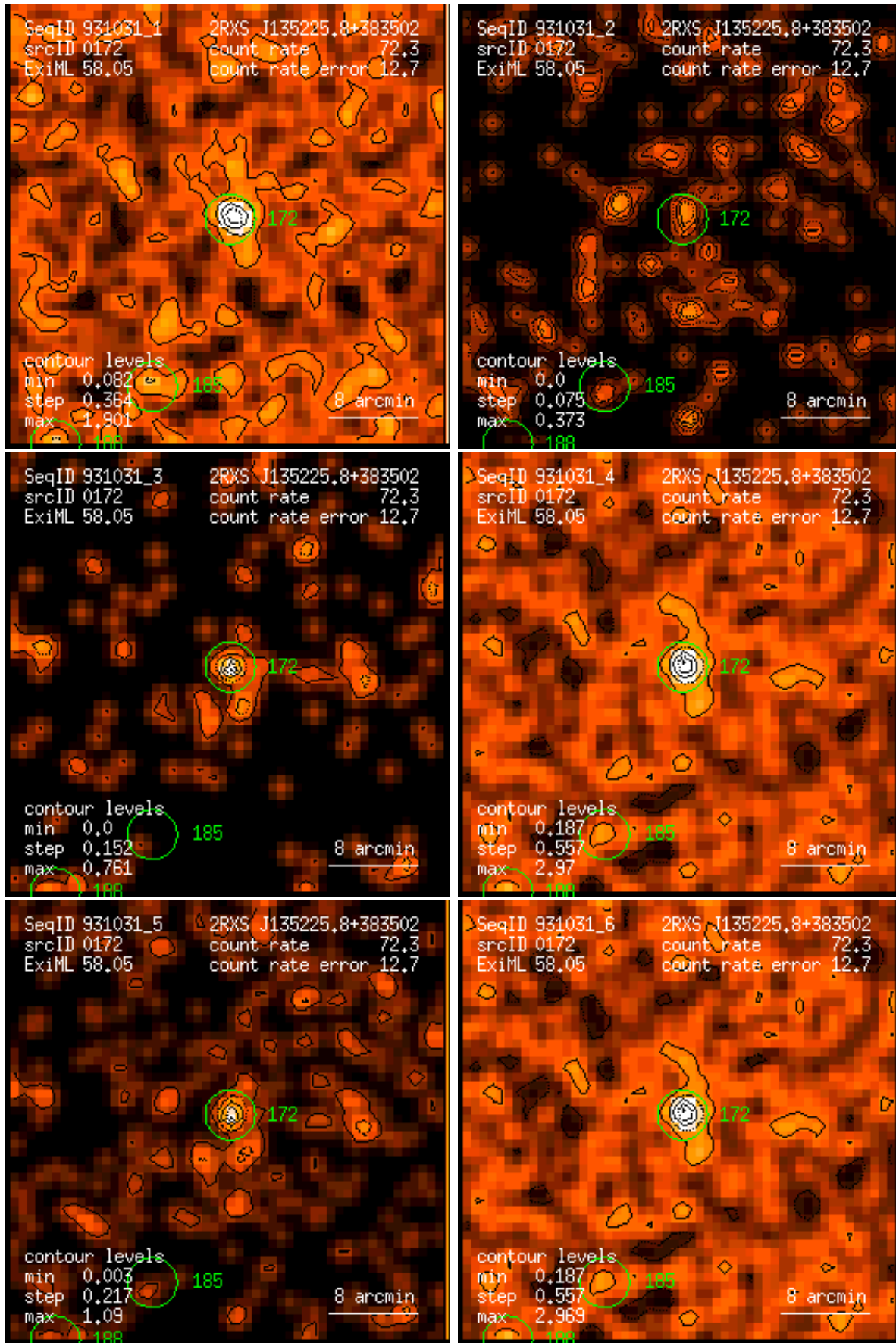
Figure 172: RASS 931031: detection 0172: band rate images, Gaussian filter: (1) PSPC channels 11 – 41, (2) 52 – 90, (3) 91 – 201, (4) 11 – 235, (5) 52 – 201, (6) 11 – 201. Broad band rates in counts/ks. Band rate contour levels in counts/ks/arcmin 2 .
